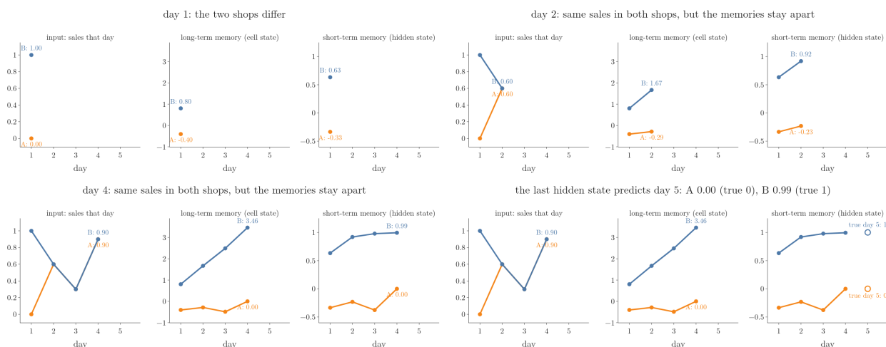
Figure 7: A one-unit LSTM reads the two sales series (left). Its long-term memory (middle) and short-term memory (right) after each day; the last short-term memory is the prediction for day 5. Idea after StatQuest, “Long Short-Term Memory (LSTM), Clearly Explained”, with our own data and trained model
