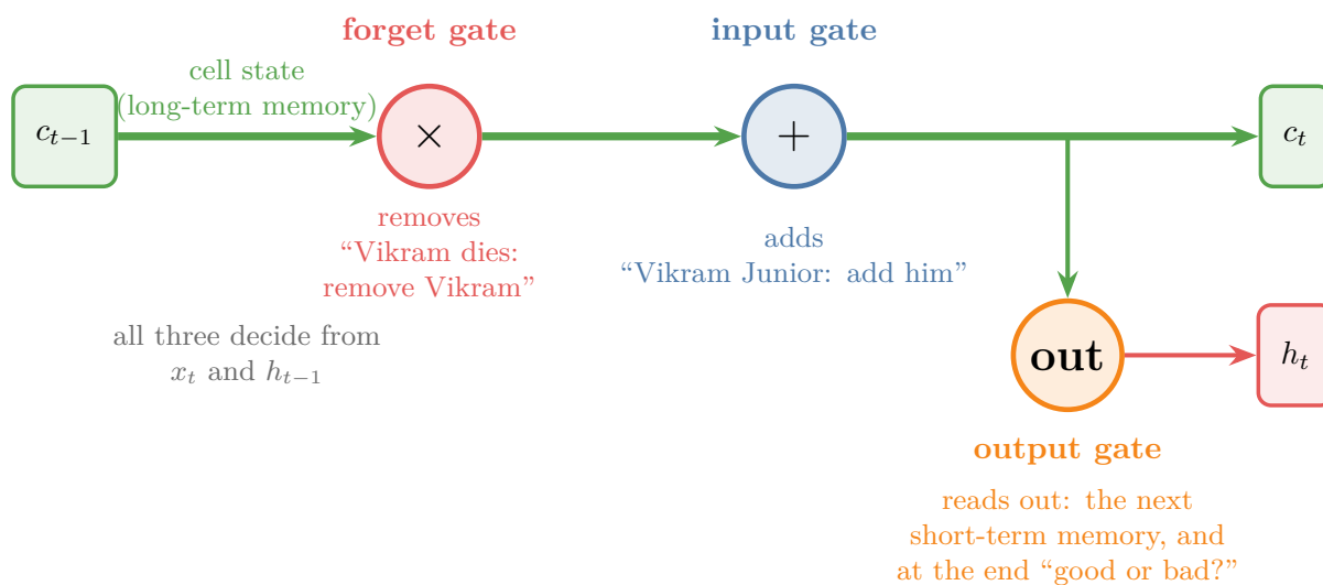
Figure 5: The three gates placed on the long-term memory. The forget gate multiplies the cell state (removes), the input gate adds to it, and the output gate reads from it to give h_t . The examples come from the story of section 4
