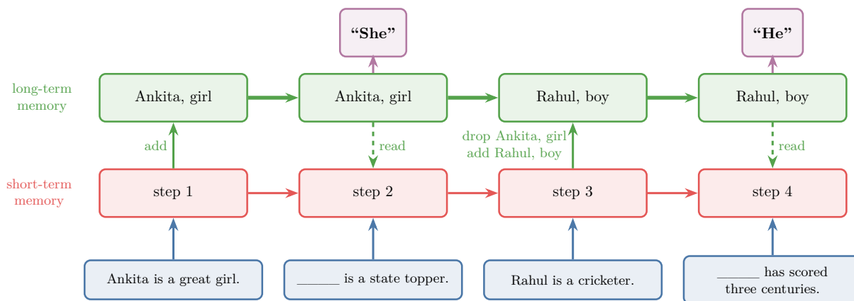
Figure 4: The pronoun example on two lanes. The short-term memory (red) reads one sentence per step; it adds “Ankita, girl” to the long-term memory (green), which carries it to the blank and gives “She”. When Rahul arrives, the long-term memory drops Ankita and stores “Rahul, boy”, which gives “He”
