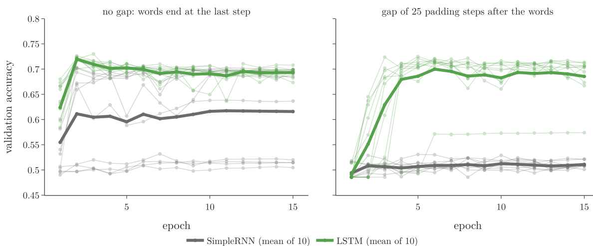
Figure 8: Validation accuracy of SimpleRNN (grey) and LSTM (green). Thin lines: 10 runs each; thick lines: their mean. The dotted line is 0.5. With 25 padding steps after the words, every SimpleRNN run stays near chance
