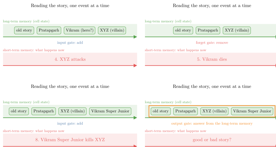
Figure 3: The story read one event at a time, with the rows of the table above. The lower lane holds what is happening now; the input gate copies what matters up to the long-term lane, and the forget gate removes what stopped mattering. The long-term lane follows Olah (2015), who draws the cell state as a line running along the top of the chain, with gates that add or remove information
