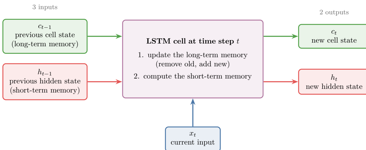
Figure 6: The LSTM cell at time step t : three inputs, two jobs, two outputs
