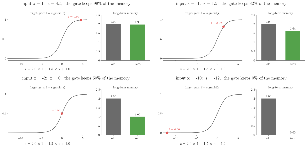
Figure 4: The forget gate of a one-unit LSTM as the input x_t falls from 1 to -10 . Left: the gate value f_t on the sigmoid curve. Right: the old long-term memory (grey, 2.00) and what the gate keeps of it (green, f_t \times 2 ). Idea after StatQuest, “Long Short-Term Memory (LSTM), Clearly Explained”, with our own numbers
