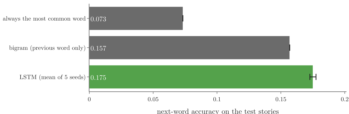
Figure 6: Next-word accuracy on the 11,366 test pairs. The LSTM bar is the mean of 5 seeds; the error bar is one standard deviation
