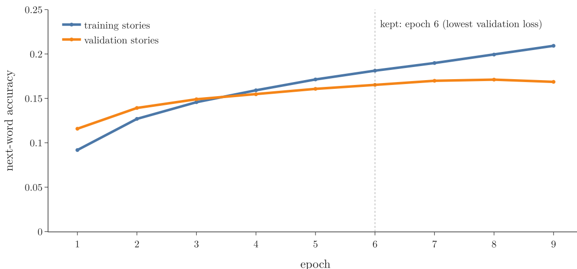
Figure 5: Next-word accuracy during training (seed 0). The dotted line marks epoch 6, the epoch with the lowest validation loss, whose weights are kept
