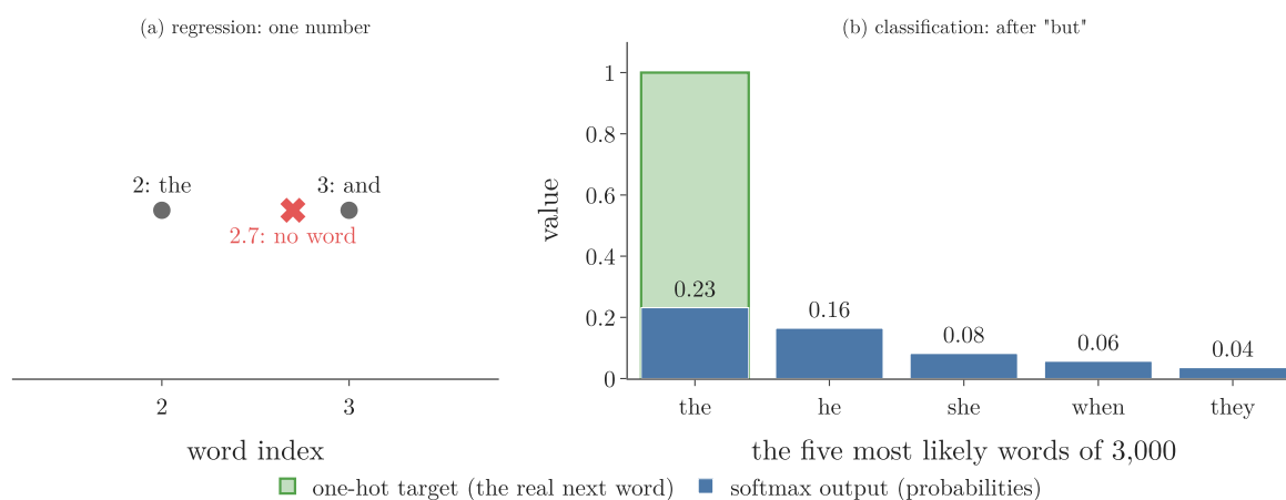
Figure 4: (a) A regression output names no word: 2.7 falls between the indices of “the” and “and”. (b) After the prefix “but”: the one-hot target (green outline, 1 for the real next word “the”) and the model’s softmax probabilities for its five most likely words (seed 0)
