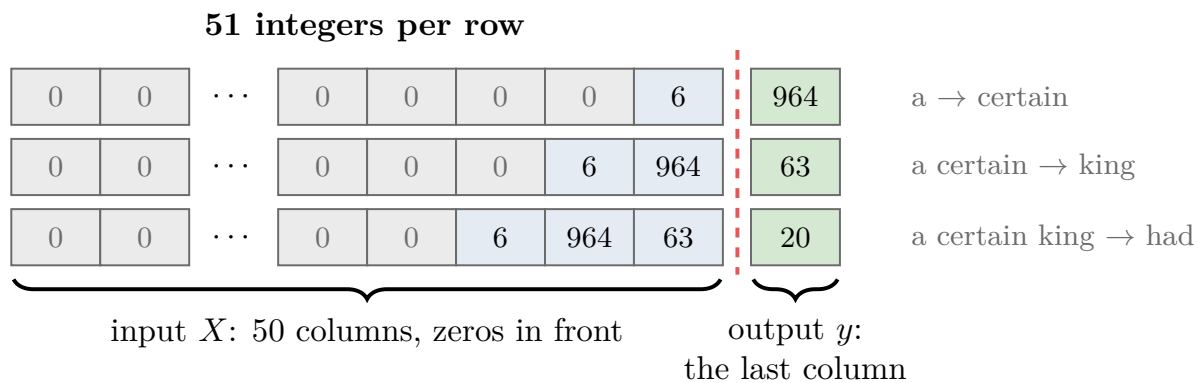
Figure 3: The first three training sequences, padded in front to 51 integers. The red dashed line splits each row: the first 50 columns are the input X , the last column is the output y
