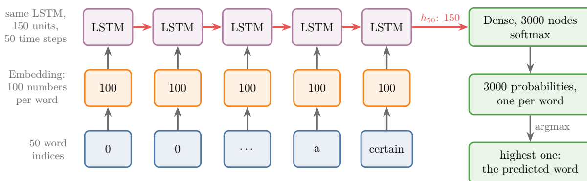
Figure 1: The next-word predictor. The words before the gap become 50 integers (zeros in front), the Embedding layer turns each into 100 numbers, the LSTM reads them one time step at a time, and its last hidden state goes to a softmax layer with one node per vocabulary word. The word with the highest probability is the prediction
