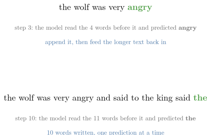
Figure 8: Text generation, one prediction per frame, for the prompt “the wolf” (seed 0). The new word (green) is appended, and the longer text is the next input
