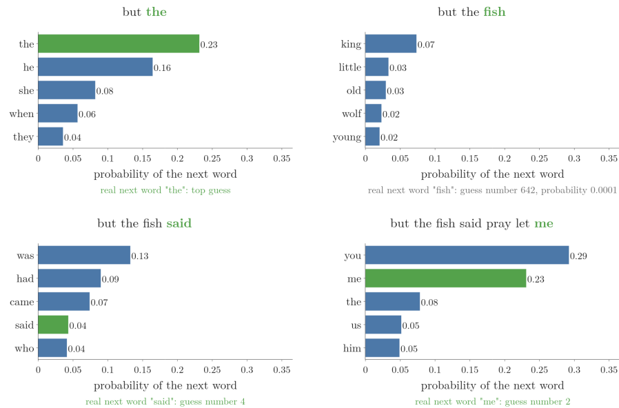
Figure 7: The sentence “But the fish said, ‘Pray let me live!’”, the first test sentence of 8 to 14 known words, typed into the model (seed 0) one word at a time. After each prefix: the model’s five most likely next words. Then the real next word appears, green when it is among the five
