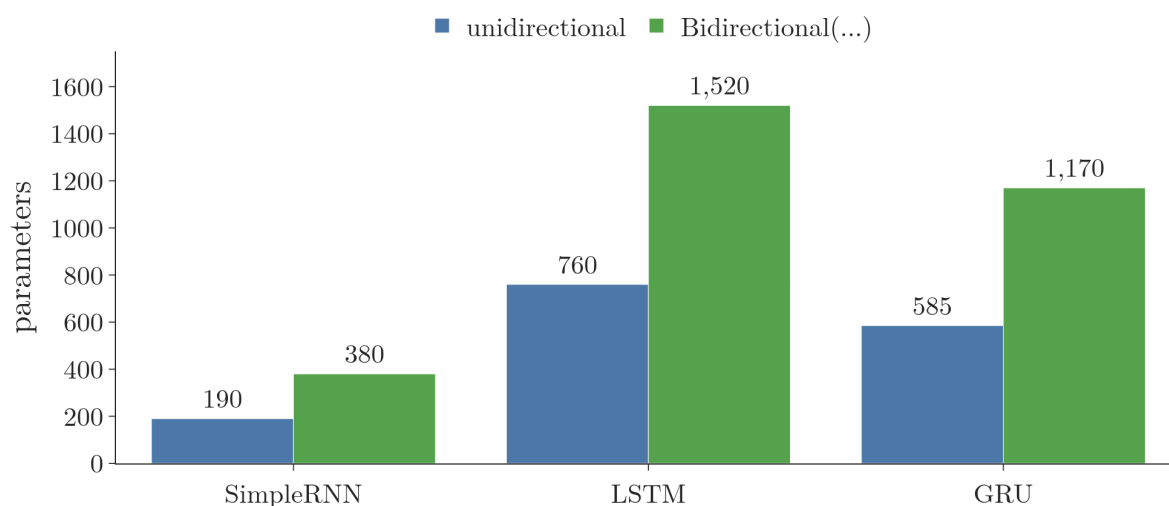
Figure 4: Parameters of a recurrent layer with 5 nodes on a 32-number input, before and after wrapping it in Bidirectional . Every bar doubles
