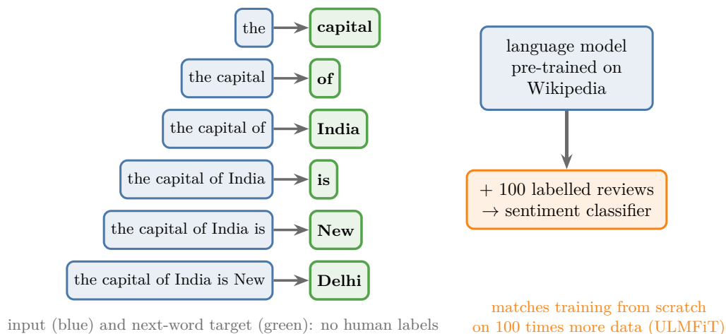
Figure 6: Left: one sentence gives six training examples for language modelling; each prefix is an input and the next word is its target, so no human labelling is needed. Right: the pre-trained model is then fine-tuned on a small labelled dataset
