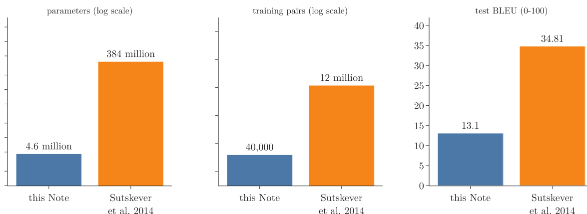
Figure 9: The Notebook’s model against the original model of Sutskever et al. (2014): parameters and training pairs (log scales: each tick up multiplies the value, it does not add to it), and test BLEU. The original’s BLEU of 34.81 comes from an ensemble of five such models
