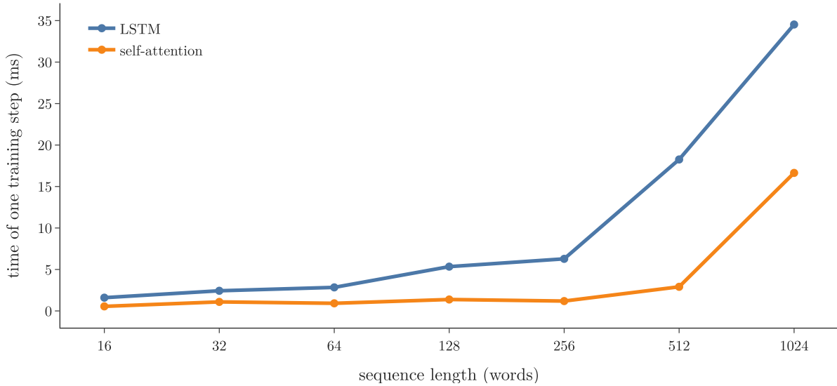
Figure 5: Time of one training step against sequence length. The LSTM’s time grows from the start; self-attention stays flat up to 256 words
