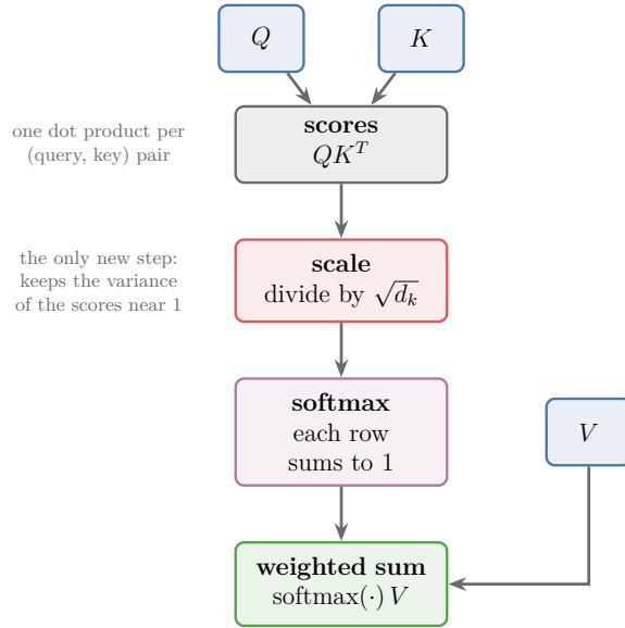
Figure 1: Scaled dot-product attention: the scores QK^T are divided by \sqrt{d_k} before the softmax. Everything else is self-attention without scaling
