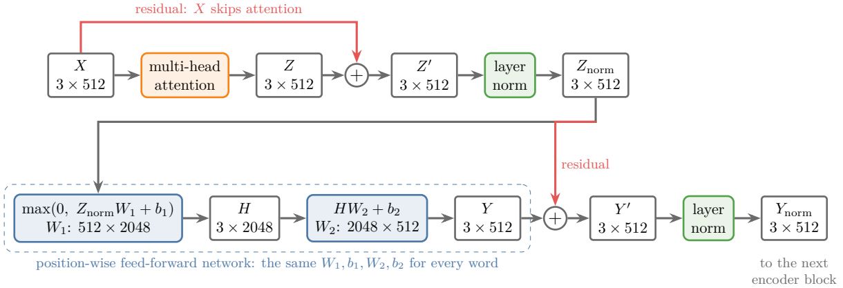
Figure 4: One encoder block for a 3-word sentence. Every matrix is 3 \times 512 except H , the hidden layer of the feed-forward network. The red arrows are the residual connections
