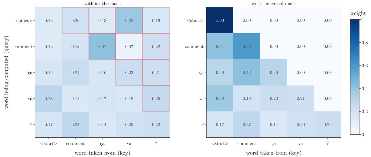
Figure 5: Self-attention weights on the decoder input. Left: without the mask, every word takes weight from the words after it (red outlines). Right: with the causal mask, every weight above the diagonal is exactly 0
