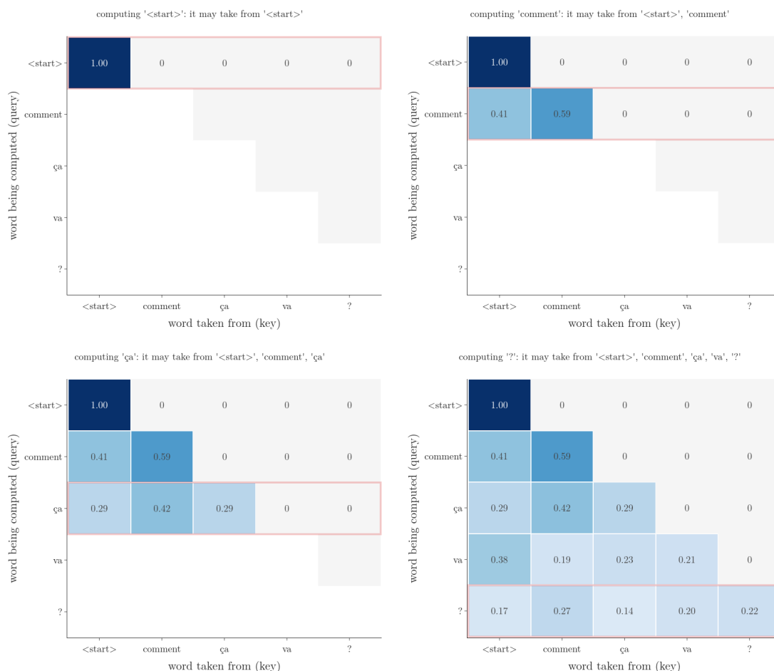
Figure 6: Masked self-attention row by row: the word being computed (red outline) may take only from itself and the words before it; the grey cells are blocked by the mask
