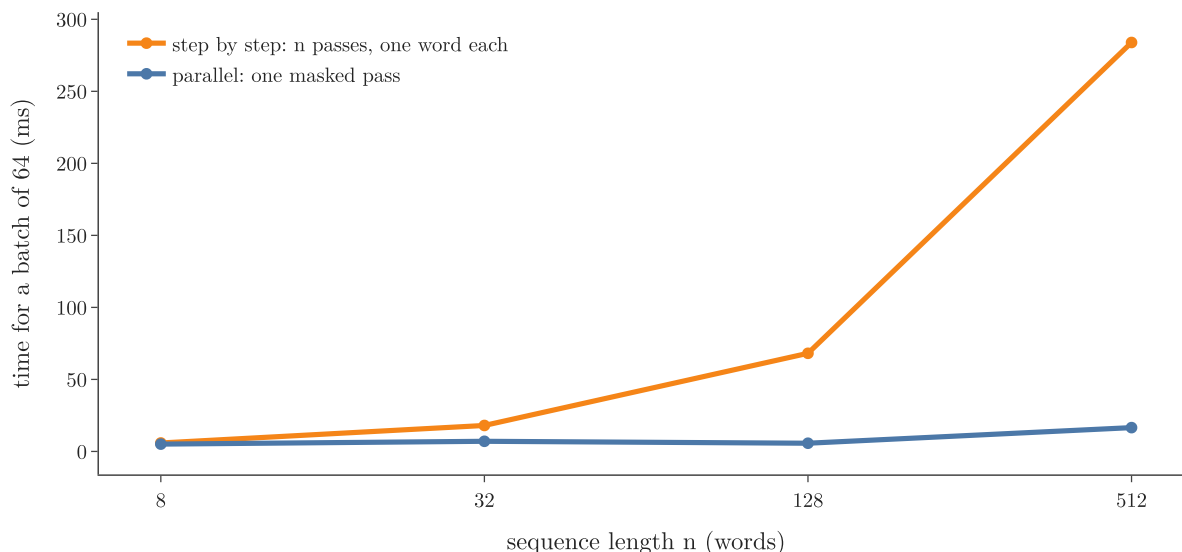
Figure 8: Time for a batch of 64: one masked pass stays nearly flat as the sequence grows, while n one-word steps grow with n
