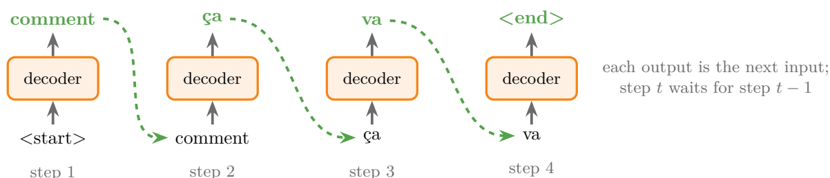
Figure 2: Autoregressive generation. At each step the decoder writes one word (green), and that word becomes part of the next step’s input (dashed), so step t must wait for step t - 1
