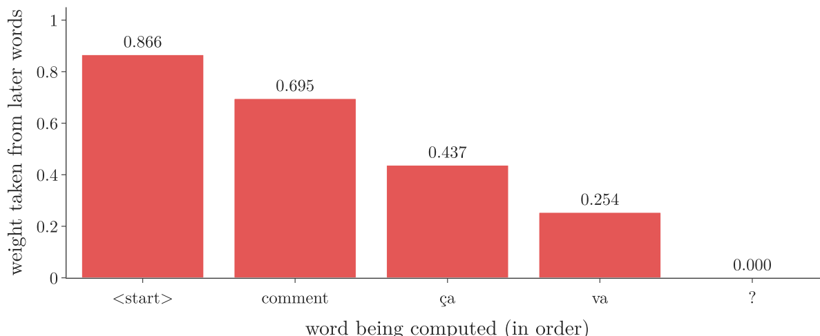
Figure 4: The last column of the table as bars: the share of each word’s weight that comes from the words after it. The earlier the word, the more of it is borrowed from the future
