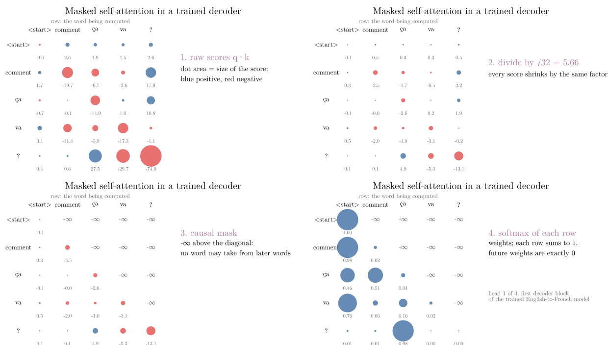
Figure 7: Masked self-attention in a trained decoder, as a grid of dots (rows: the word being computed). Raw scores q \cdot k (blue positive, red negative), divided by \sqrt{d_k} , masked with -\infty above the diagonal, then the softmax of each row
