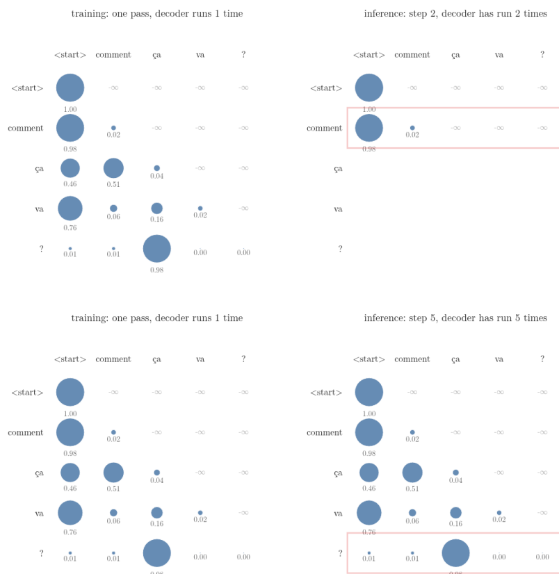
Figure 3: Training against inference, with the masked weights of a trained decoder (one attention head, first decoder block). Left: training computes every row in one pass. Right: inference computes one new row per step (red outline), as each word is written. The rows are the same numbers
