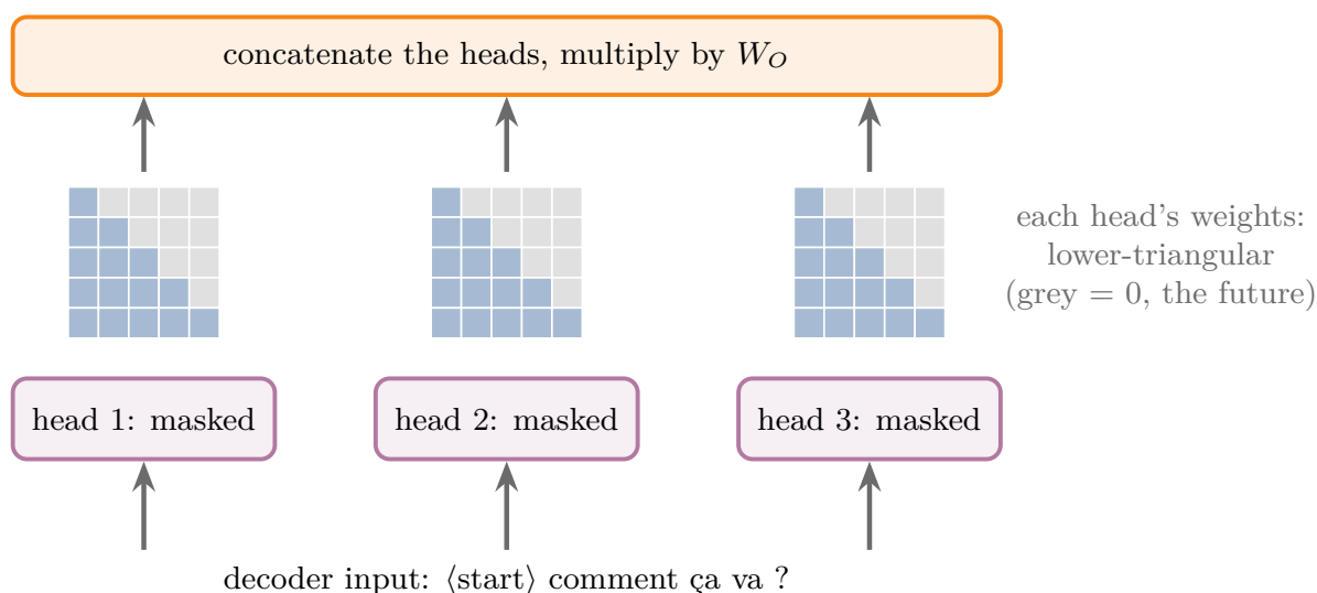
Figure 9: Masked multi-head attention. Every head applies the causal mask, so every head’s weight matrix is lower-triangular (grey: the blocked future); the heads are then concatenated and multiplied by W_O
