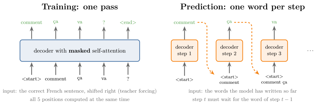
Figure 1: Left: during training the decoder receives the whole correct French sentence, shifted right, and computes every position in one pass. Right: during prediction it writes one word per step, and each step must wait for the word of the step before
