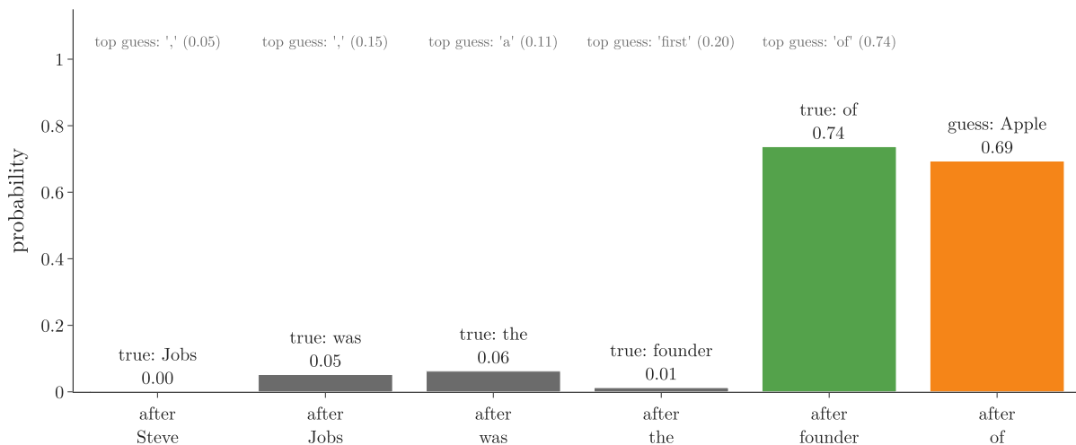
Figure 7: The table as bars: the probability the pass gave the true next token at each position (green when it was also the top guess), with the top guess above. At the last position there is no true token yet; the orange bar is the guess used for generation
