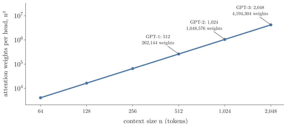
Figure 8: Attention weights computed by one head for a context of n tokens: n^2 , on log scales (up the vertical axis each gridline is ten times the one below; along the horizontal axis each tick is double the one before). Each doubling of the context, as from GPT-1 to GPT-2 to GPT-3, multiplies them by 4
