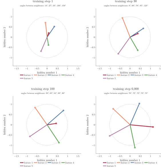
Figure 8: Training the toy model with 5 equally important features, each active 5 percent of the time, in 2 hidden numbers. The 5 directions spread into a pentagon
