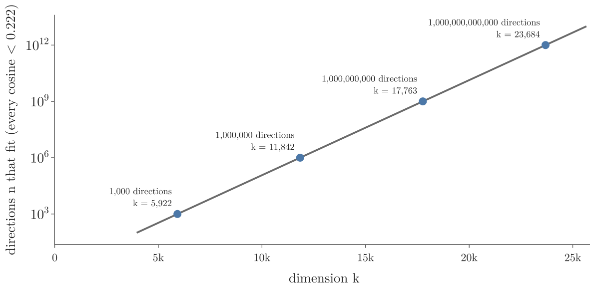
Figure 5: The Johnson–Lindenstrauss guarantee with \varepsilon = 0.1 : the number of directions that fit, every cosine below 0.222, against the dimension. On a log scale the line is straight: the count grows exponentially with the dimension
