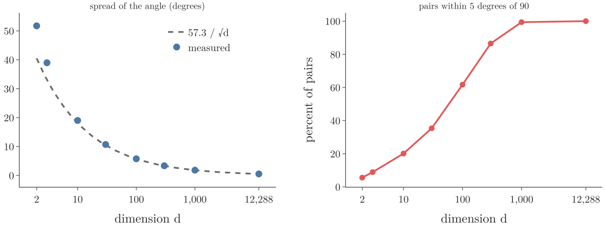
Figure 3: Left: the measured spread of the angle between random directions (dots) against the prediction 57.3/\sqrt{d} (dashed). Right: the share of pairs within 5 degrees of perpendicular rises from 6 percent in 2 dimensions to 100 percent in 12,288
