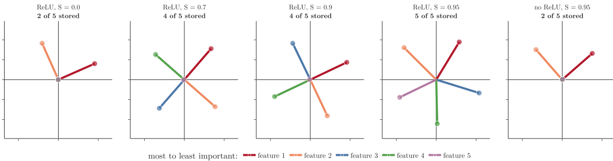
Figure 7: Toy model of superposition: the 2-number direction of each of 5 features after training, as features get sparser. Last panel: no ReLU
