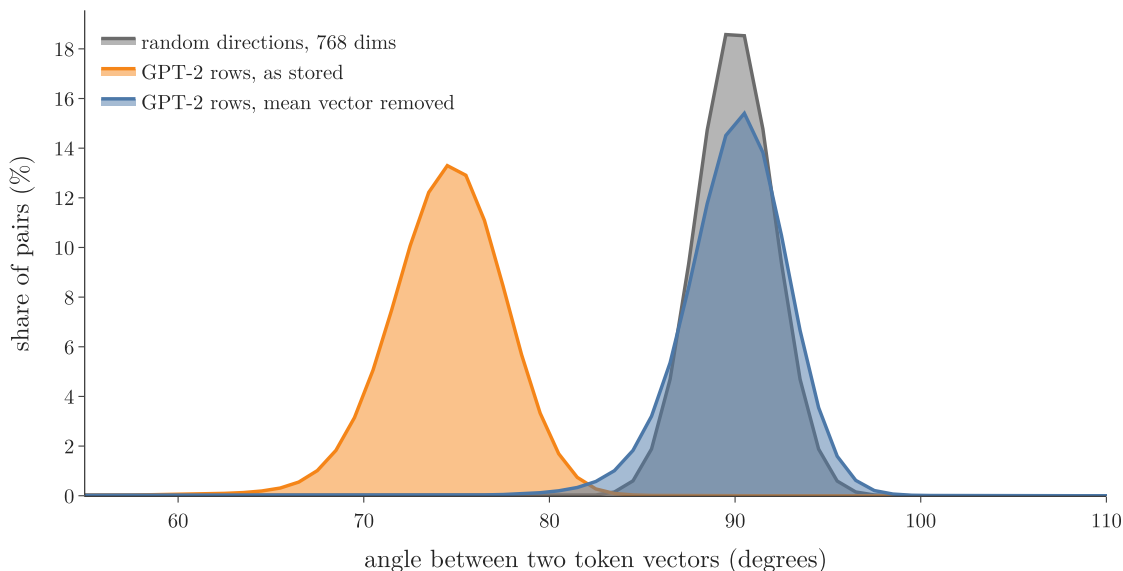
Figure 6: Angles between 3,000 token vectors of GPT-2 small. Orange: as stored. Blue: after subtracting the mean of all 50,257 token vectors. Grey: random directions in 768 dimensions
