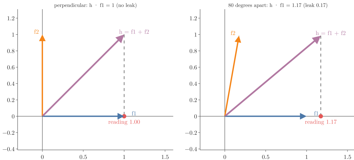
Figure 2: An example of our own: two features, both with strength 1, so h = f_1 + f_2 . Reading feature 1 with h \cdot f_1 projects h onto f_1 (dashed). Left: perpendicular directions give exactly 1. Right: directions 80 degrees apart give 1 + \cos 80^\circ = 1.17 ; the extra 0.17 is the leak from feature 2
