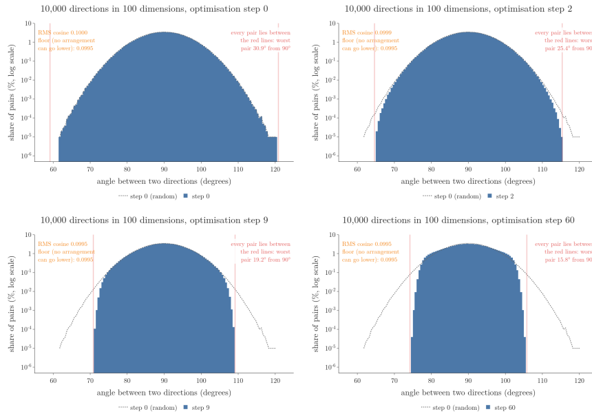
Figure 4: 10,000 directions in 100 dimensions, nudged to be more perpendicular. Dotted grey: the random start. Red lines: every pair lies between them. The log scale shows the rare pairs far from 90 degrees
