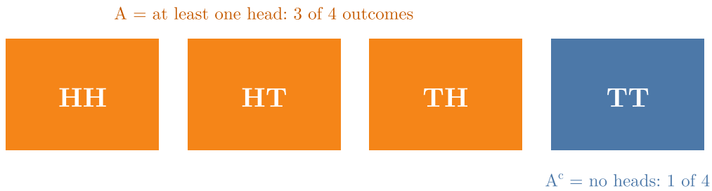
Figure 6: The two-toss sample space split into A = at least one head (orange, 3 outcomes) and its complement, no heads (blue, 1 outcome).
