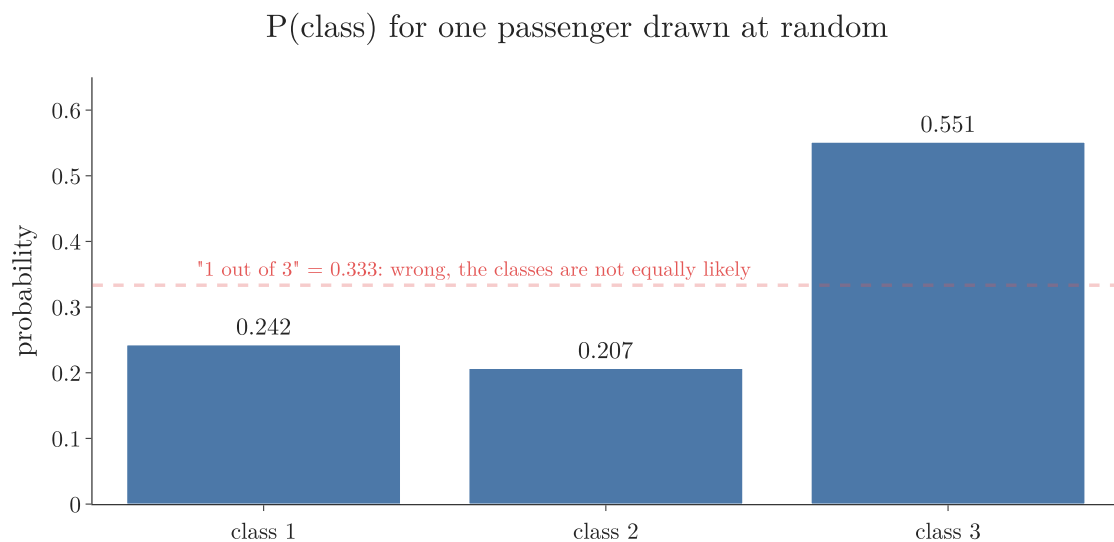
Figure 3: The empirical probability of each Titanic class, from 891 passengers, against the wrong “1 out of 3” (dashed).
