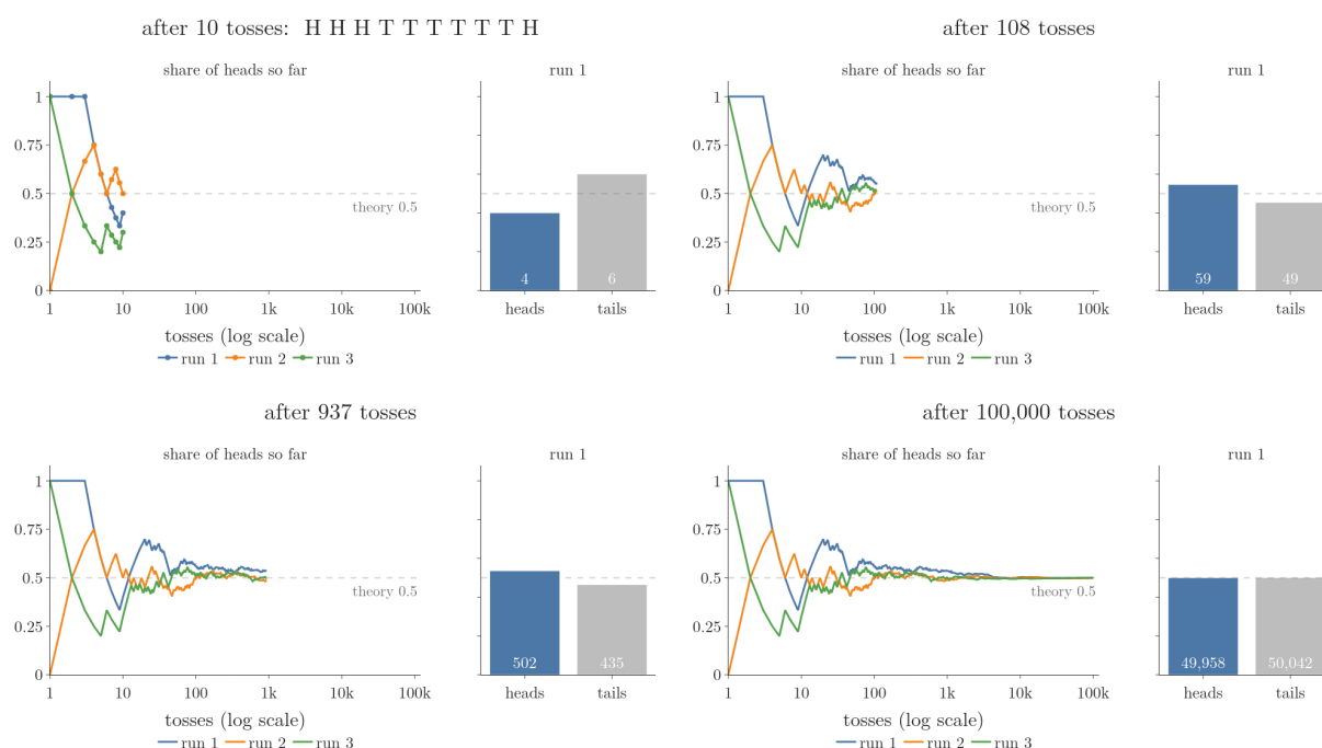
Figure 1: A fair coin tossed up to 100,000 times in three runs: the share of heads so far (left) and run 1's head and tail counts (right) settle on the theoretical 0.5
