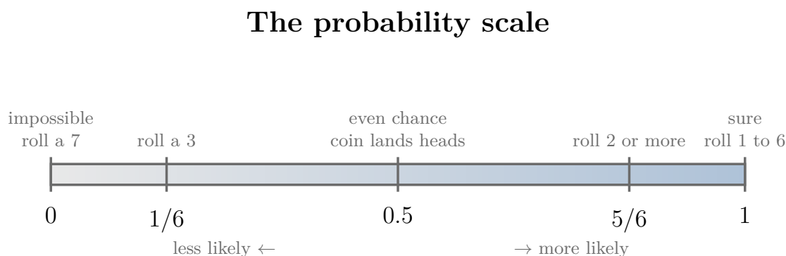
Figure 2: The probability scale from 0 (impossible) to 1 (sure)
