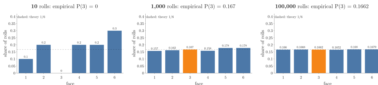
Figure 5: The share of each face in 10, 1,000 and 100,000 simulated rolls of a die (the Notebook's draws), against the theoretical 1/6 (dashed). Face 3 is orange.
