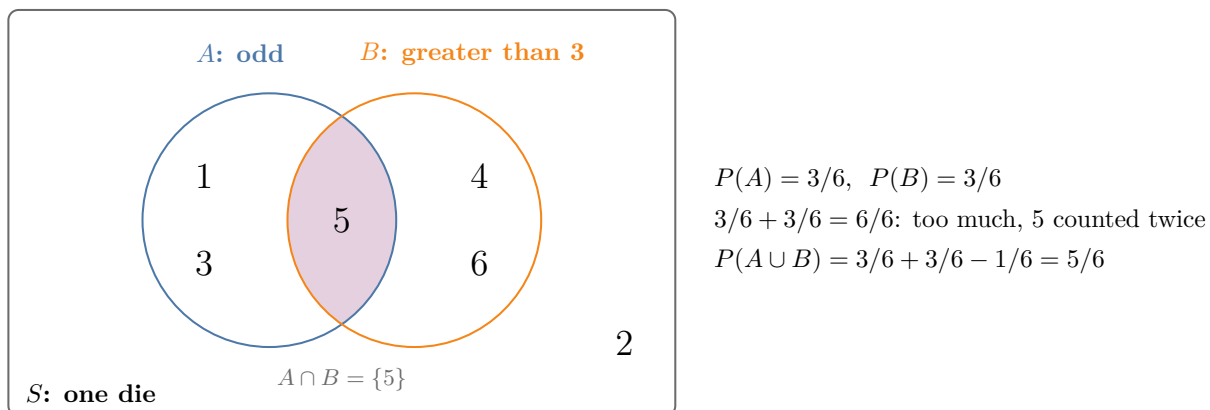
Figure 7: The general addition rule on one die: the overlap \{5\} is counted twice by P(A) + P(B)
