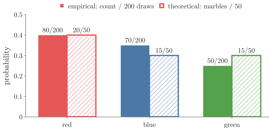
Figure 4: The marble bag: empirical shares from 200 draws (solid) against the theoretical shares from the bag’s contents (hatched)
