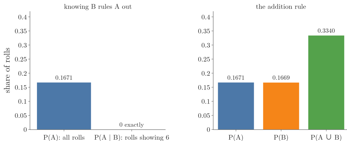
Figure 2: One million rolls of a fair die. Left: the share showing 3 is 0.1671 over all rolls, and exactly 0 among the rolls that showed 6. Right: the shares of 3, of 6, and of “3 or 6”, which is their sum, about 1/3 .
