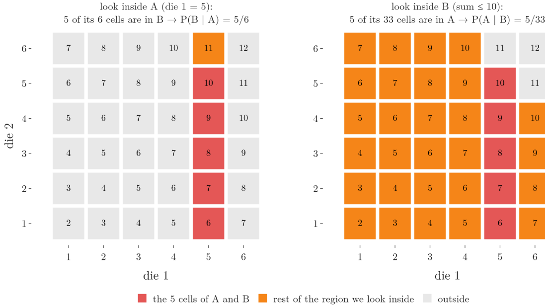
Figure 3: The proof on the 36 outcomes of two dice. Left: inside A, 5 of 6 cells are in B, so P(A \cap B) = 5/6 \times 6/36 . Right: inside B, 5 of 33 cells are in A, so P(A \cap B) = 5/33 \times 33/36 . Both equal 5/36
