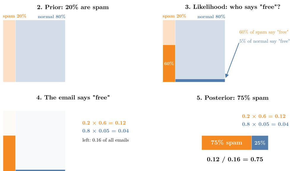
Figure 5: Bayes’ theorem as areas, on the spam numbers. Prior: a 20% spam strip. Likelihood: the “free” share inside each strip. Evidence: only the two dark pieces remain (0.12 and 0.04). Posterior: rescaled to fill the whole, spam is 0.12 / 0.16 = 75\% . Idea after Sanderson (3Blue1Brown), “Bayes theorem, the geometry of changing beliefs”.
