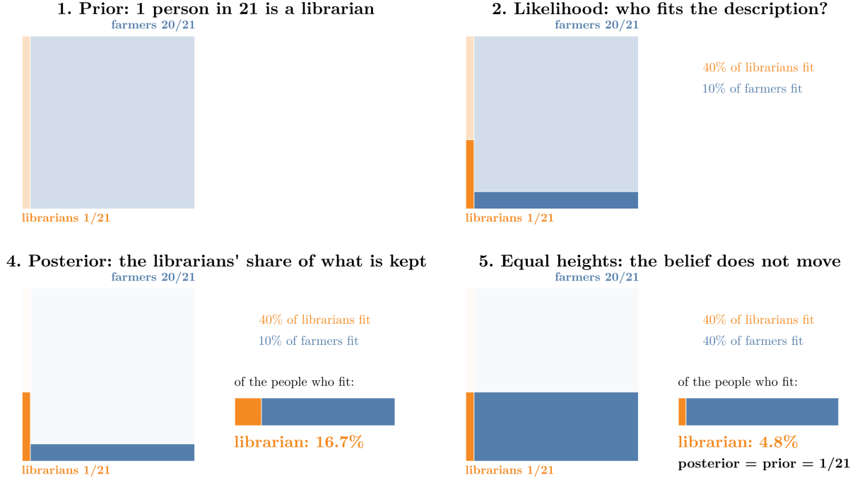
Figure 4: Bayes' theorem as areas, on the librarian numbers. The librarians are a strip of width 1/21 . The description keeps 40% of that strip and 10% of the farmers' strip. The bar on the right shows the librarians' share of what is kept: 16.7%. In the last step the farmers' height rises to 40%, and the share falls back to the prior, 4.8%. Idea after Sanderson (3Blue1Brown), "Bayes theorem, the geometry of changing beliefs".
