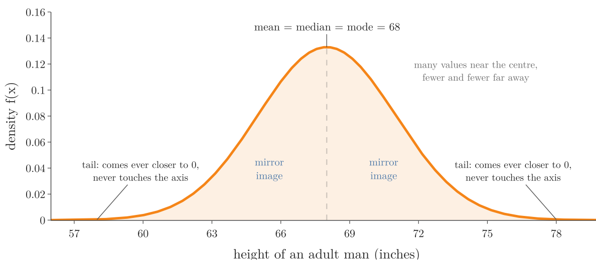
Figure 1: The normal curve of adult men's heights: mean 68 inches, standard deviation 3 inches
