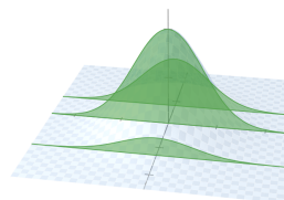
Figure 5: The bell lifted to a round bell-shaped surface: its volume by thin cylindrical shells is pi, by slices it is C^2 , so C = square root of pi (idea after 3Blue1Brown, “Why \pi is in the normal distribution (beyond integral tricks)”)
