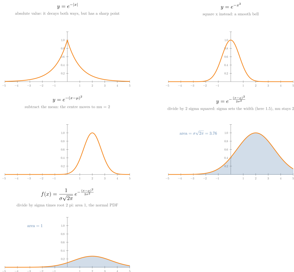
Figure 4: Building the normal PDF term by term: the bell, the shift, the width, the area
