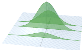
Figure 5: The bell lifted to a round bell-shaped surface: its volume by thin cylindrical shells is pi, by slices it is C^2 , so C = square root of pi (idea after 3Blue1Brown, “Why \pi is in the normal distribution (beyond integral tricks)”)
