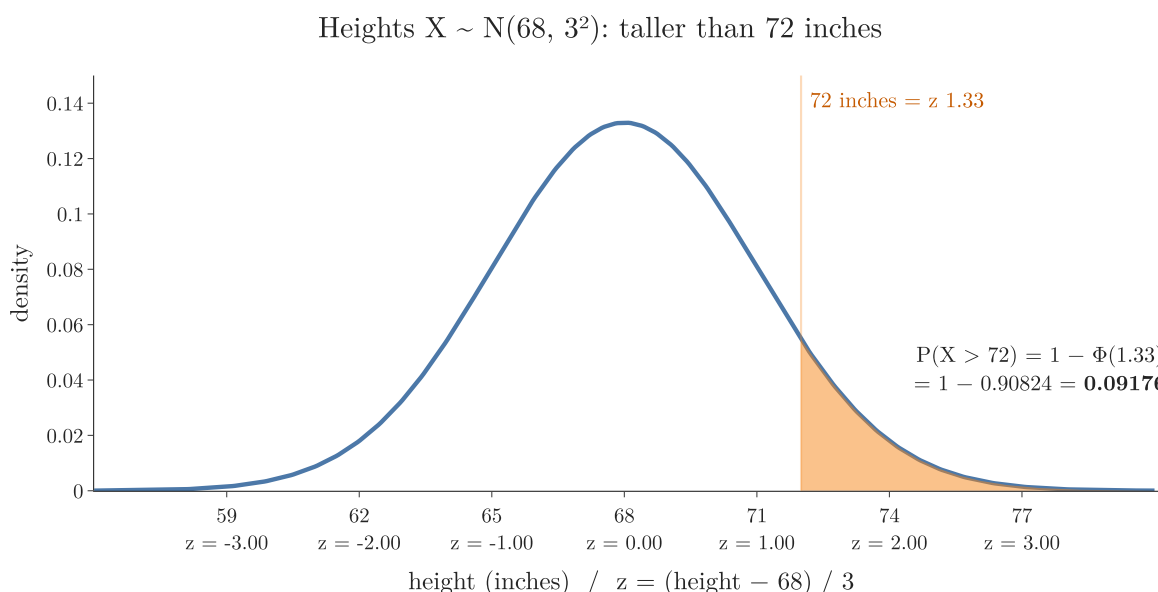
Figure 5: Heights N(68, 3^2) . The area above 72 inches (orange) is 1 - \Phi(1.33) = 0.09176 ; the tick labels give each height's z-score.
