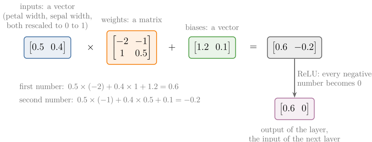
Figure 3: One layer of a neural network on one iris flower: the input vector times the weight matrix, plus the bias vector, then ReLU. Worked example after StatQuest, “Essential Matrix Algebra for Neural Networks”, with our own numbers.
