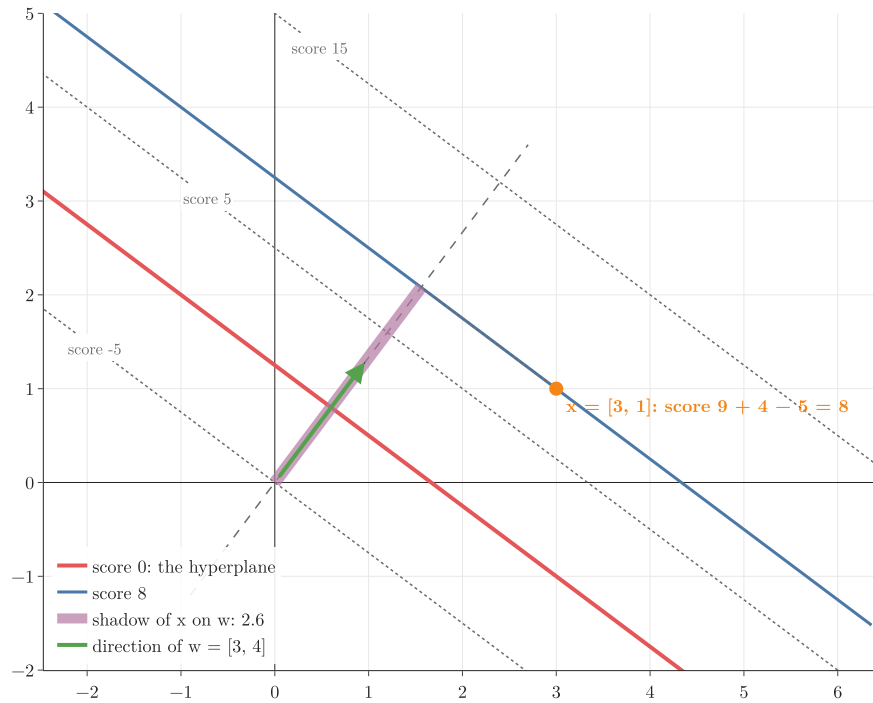
Figure 7: The score of a linear model with w = [3, 4] and shift -5: every line perpendicular to w is a line of equal score
