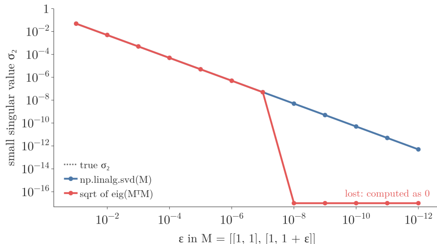
Figure 9: The small singular value of M as \varepsilon shrinks: np.linalg.svd (blue) follows the true value (dotted, under the blue line); the square root of the eigenvalue of M^T M (red) drops to 0 from \varepsilon = 10^{-8} on
