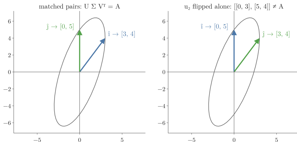
Figure 4: Left: the matched factors rebuild A . Right: the same factors with only \mathbf{u}_2 flipped. The ellipse is identical, but \hat{i} and \hat{j} (the unit arrows along x and y , [1, 0] and [0, 1] ) land in swapped places
