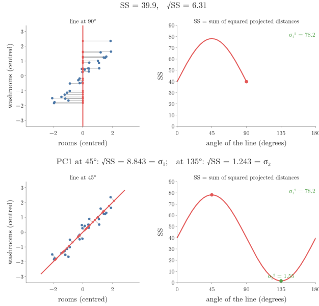
Figure 2: A line through the centre of the 30 centred flats turns from 0^\circ to 180^\circ . Each flat drops onto it (red feet); the right panel traces SS, the sum of the squared distances of the feet from the centre. The peak, \sigma_1^2 = 78.2 at 45^\circ , is PC1. Idea after StatQuest, “Principal Component Analysis (PCA), Step-by-Step”
