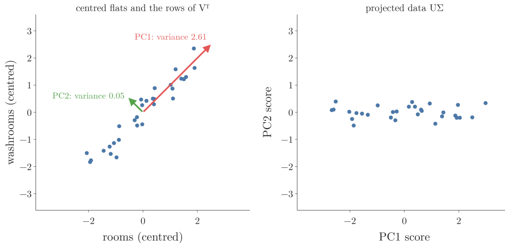
Figure 3: Left: the 30 centred flats with the two rows of V^T drawn as arrows (length two standard deviations along each). Right: the same flats as rows of U\Sigma
