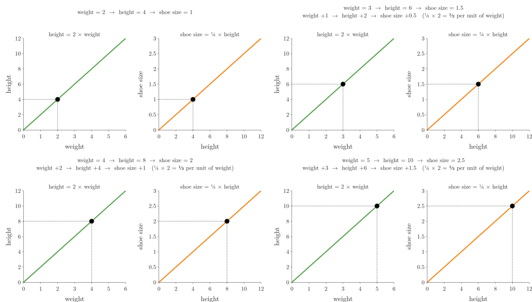
Figure 8: Two lines chained together: \text{height} = 2 \times \text{weight} (left) and \text{shoe size} = \frac{1}{4} \times \text{height} (right). As the weight moves from 2 to 5, the height moves twice as far and the shoe size half as far as the weight: \frac{1}{4} \times 2 = \frac{1}{2} . Numbers after StatQuest, “The Chain Rule, Clearly Explained!!!”
