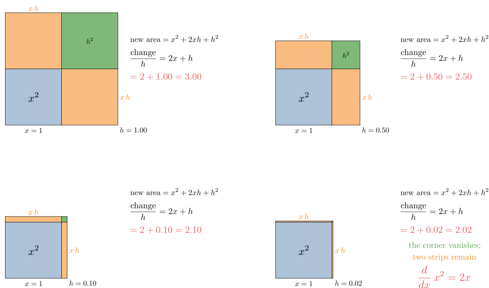
Figure 5: A square of side x = 1 grows by h . The new area is two orange strips of area xh and a green corner h^2 , so the change divided by h is 2x + h . Key frames: h = 1, 0.5, 0.1 , and the limit
