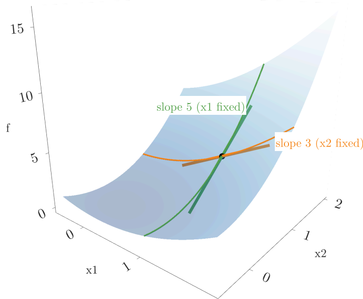
Figure 5: The surface f(x_1, x_2) = x_1^2 + x_1x_2 + 2x_2^2 cut along x_2 = 1 (orange) and along x_1 = 1 (green); the thick lines are the tangent lines at (1, 1)
