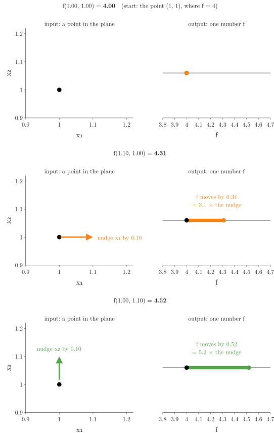
Figure 4: The point (1, 1) in the input plane (left) and the single output number f on a number line (right). A nudge of 0.1 in x_1 alone moves the output by 0.31; the same nudge in x_2 alone moves it by 0.52. Idea after Khan Academy, “Partial derivatives, introduction”
