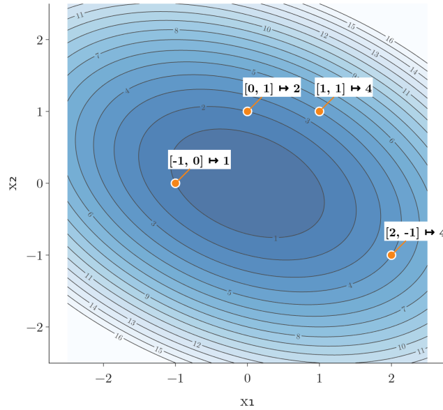
Figure 3: The running example on a contour map, with four input vectors and the single number the function returns for each. [1, 1] and [2, -1] both give 4 and lie on the same contour line.
