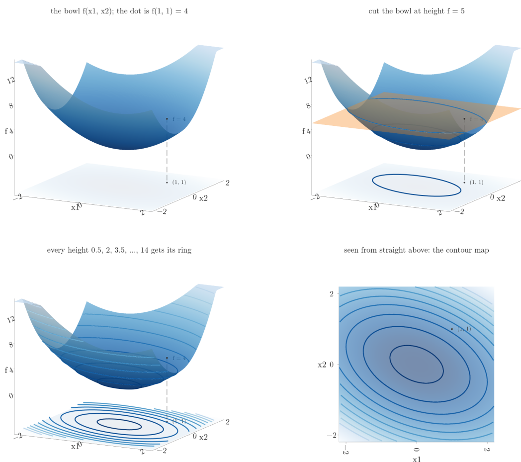
Figure 1: How a contour map is made. The bowl f(x_1, x_2) = x_1^2 + x_1x_2 + 2x_2^2 is cut by horizontal planes; each cut is a ring of equal height that drops to the floor; the camera then tilts from the side to straight above, and the floor becomes the contour map of Figure 2. Darker blue = lower. Black dot: (1, 1) , where f = 4 . Our own animation
