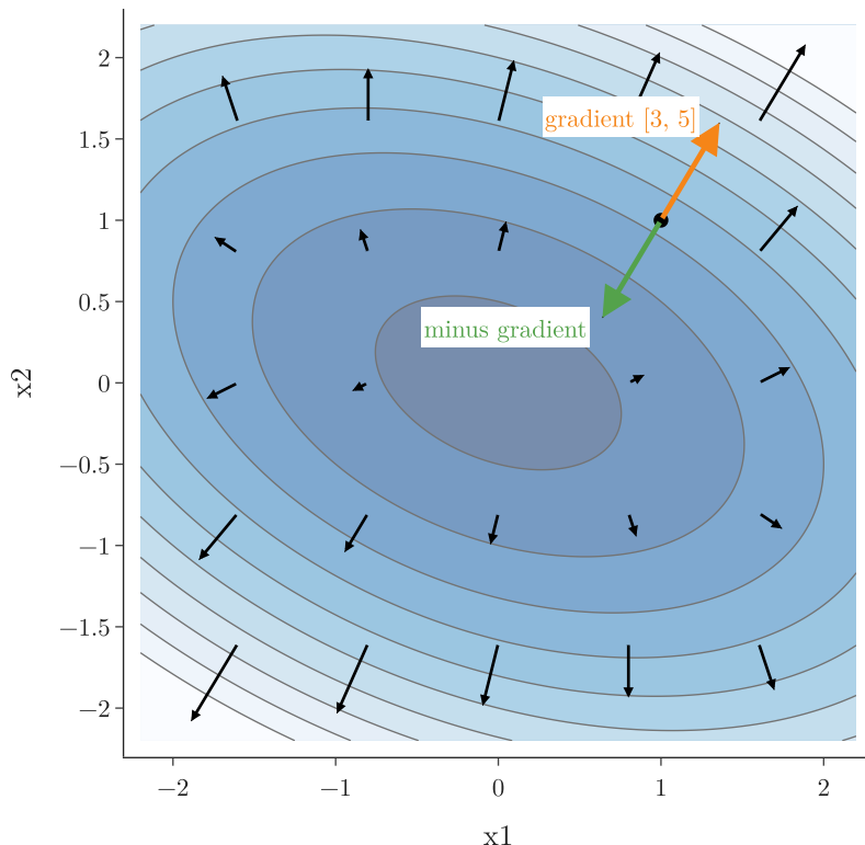
Figure 2: Contour map of f(x_1, x_2) = x_1^2 + x_1x_2 + 2x_2^2 with gradient arrows: each crosses the contour lines at right angles and points uphill
