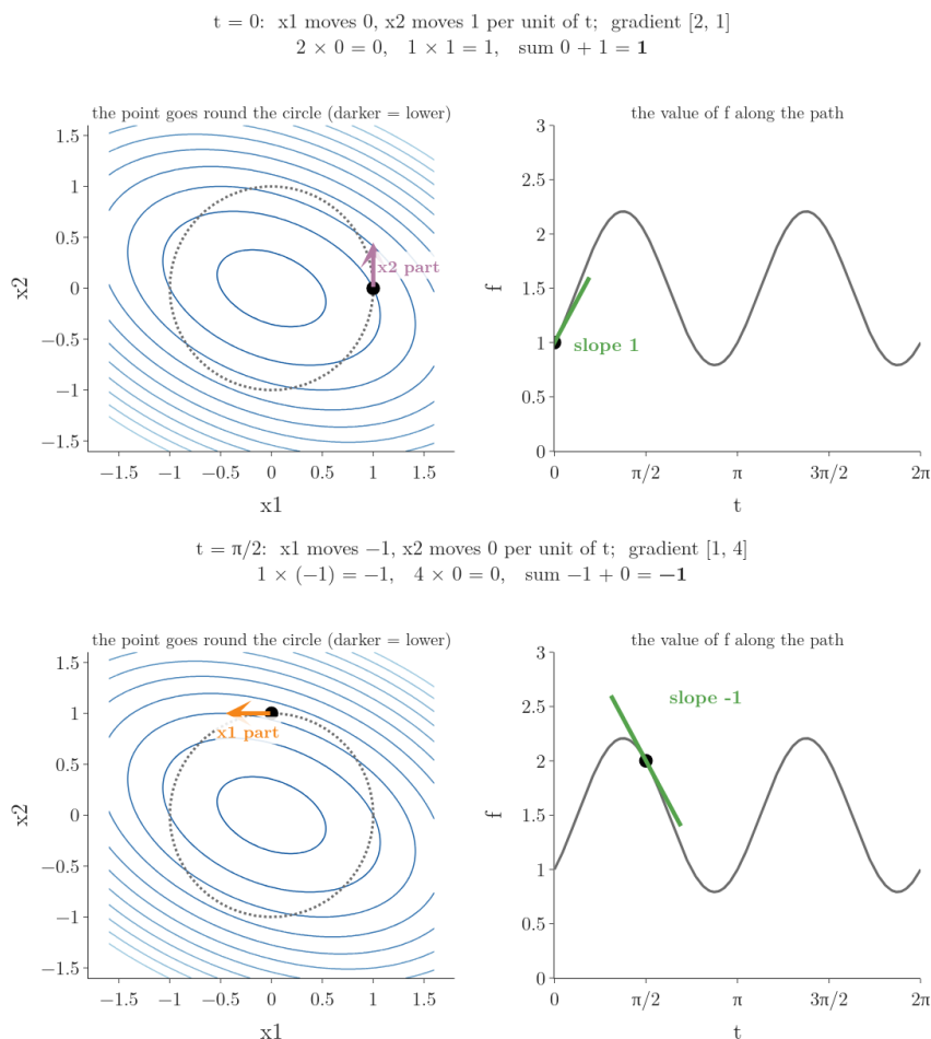
Figure 11: A point goes round the unit circle on the contour map of the bowl (left); the right panel tracks the value of f . At t = 0 the step is all along x_2 (purple) and f rises with slope 1; at t = \pi/2 it is all along x_1 (orange) and f falls with slope -1 . Idea after Khan Academy, “Multivariable chain rule” and “Multivariable chain rule intuition”; our own function
