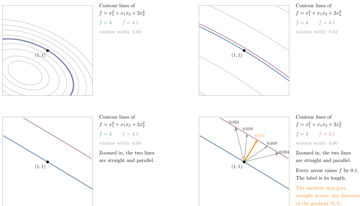
Figure 7: Zooming in on (1, 1) : the contour lines f = 4 (blue) and f = 4.1 (purple) become straight and parallel. Of the arrows that raise f by 0.1, the shortest (orange, length 0.017) crosses at a right angle and points along the gradient [3, 5] . Idea after Khan Academy, “Gradient and contour maps”; our own function
