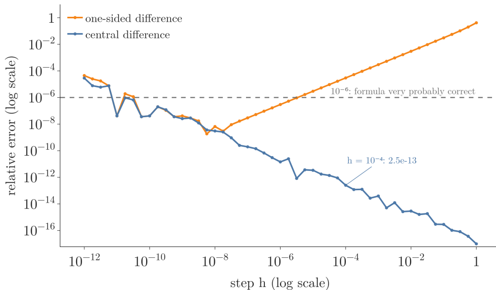
Figure 12: Relative error of the numerical gradient against the step h , on the three-point loss at m = 1 , b = 0 . Orange: one-sided difference, error shrinking with h until rounding takes over. Blue: central difference, exact for this quadratic loss except for rounding, which grows as h shrinks. Dashed: the 10^{-6} threshold.
