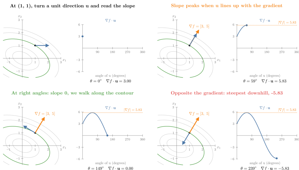
Figure 8: At (1, 1) a unit direction \mathbf{u} turns full circle (left); the slope \nabla f \cdot \mathbf{u} is traced against its angle (right): 3 along the x_1 -axis, a peak of 5.83 when \mathbf{u} lines up with \nabla f = [3, 5] , 0 along the contour line, -5.83 straight downhill
