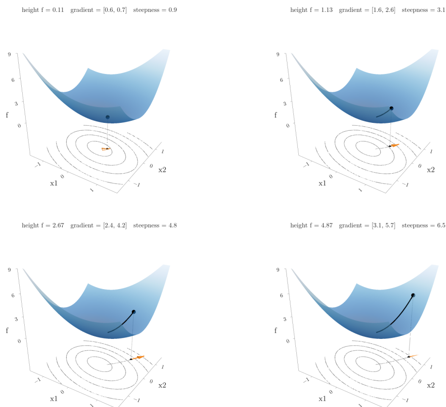
Figure 6: A hiker (black dot) climbs the bowl by always stepping along the gradient arrow (orange) drawn on the contour map below. The dashed shadow of the path crosses every contour line at a right angle, and the arrow grows as the surface gets steeper. Idea after Khan Academy, “Gradient and graphs”; our own function
