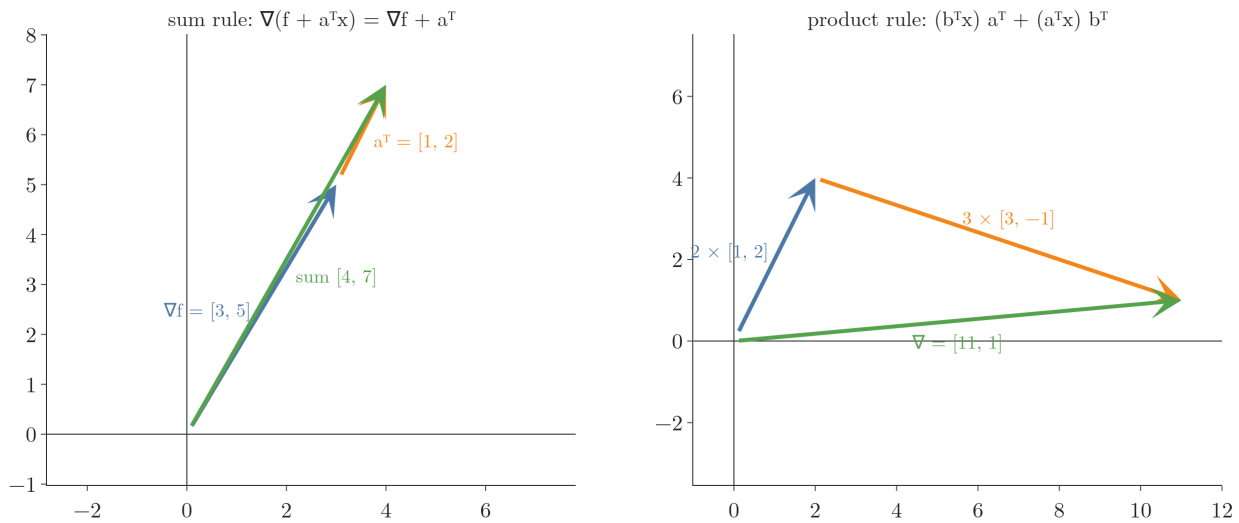
Figure 9: Gradient rules as additions of arrows at \mathbf{x} = (1, 1) . Left, sum rule: the gradient of f + \mathbf{a}^\top \mathbf{x} is \nabla f = [3, 5] plus \mathbf{a}^\top = [1, 2] , giving [4, 7] . Right, product rule: 2 \times [1, 2] plus 3 \times [3, -1] gives the gradient [11, 1] .
