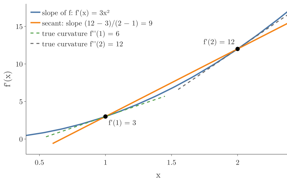
Figure 11: The secant idea for f = x^3 : the line through the slope readings at x = 1 and x = 2 has slope 9, a stand-in for the true curvatures 6 and 12
