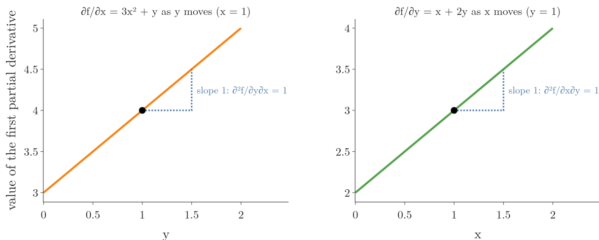
Figure 4: Mixed partial derivatives of f(x, y) = x^3 + xy + y^2 near (1, 1) . Left: the x -slope 3x^2 + y as y moves, with x = 1 fixed: slope 1. Right: the y -slope x + 2y as x moves, with y = 1 fixed: also slope 1.
