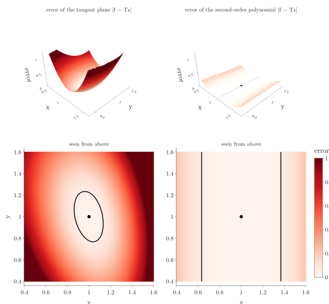
Figure 3: The size of the error near (1, 1) , on the same colour scale. Top: each error as a surface (height = error). Bottom: the same seen from above as a heat map. Left: the tangent plane, |f - T_1| . Right: the second-order Taylor polynomial, |f - T_2| . The black line marks an error of 0.05; the region inside it is about nine times larger for T_2 .
