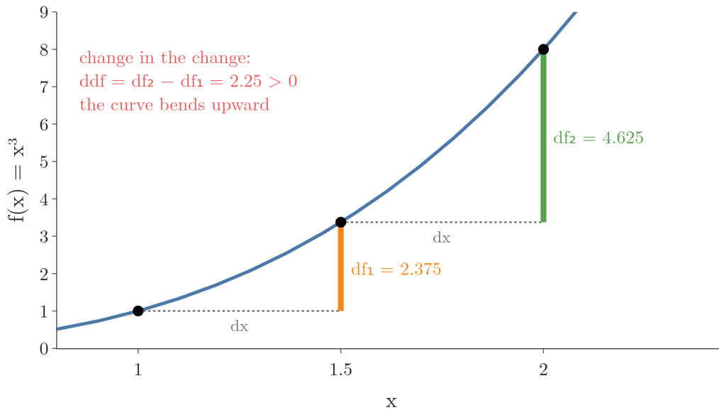
Figure 2: The second derivative as the change in the change, for f(x) = x^3 from x = 1 . Two equal steps (drawn large, dx = 0.5 ) raise f by 2.375 and then by 4.625; the second rise is bigger, so the curve bends upward. Idea after 3Blue1Brown, “Higher order derivatives”
