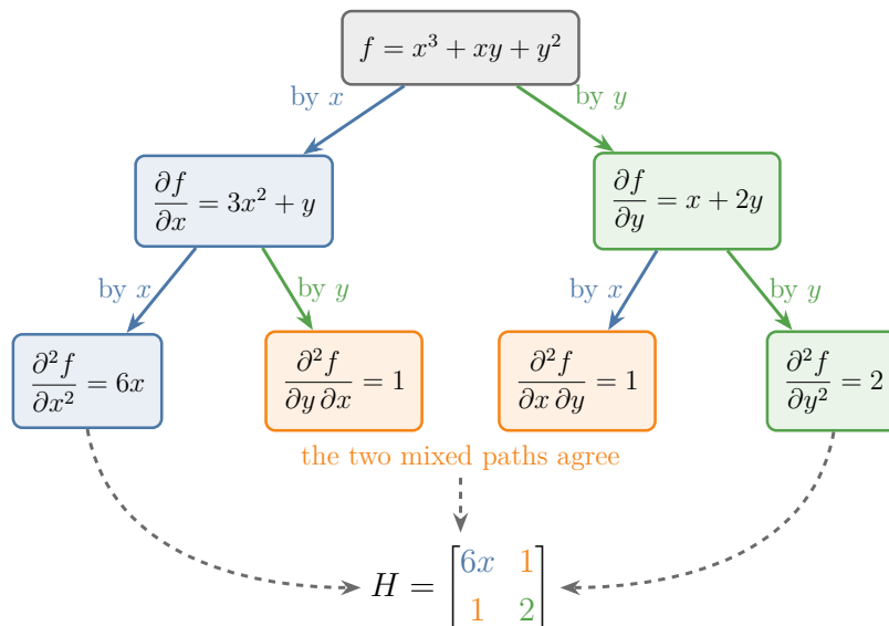
Figure 5: The tree of derivatives of f = x^3 + xy + y^2 . Two differentiations give four second partial derivatives; the two mixed paths agree. The four results fill the Hessian. Idea after Khan Academy, “Symmetry of second partial derivatives” and “The Hessian matrix”; our own function
