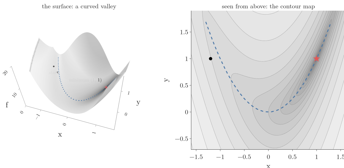
Figure 12: The curved valley f(x, y) = (1 - x)^2 + 5(y - x^2)^2 as a surface (left) and seen from above as a contour map (right). Same colours (darker = lower), same square. Black dot: the start (-1.2, 1) ; red: the minimum (1, 1) ; dashed: the valley floor y = x^2
