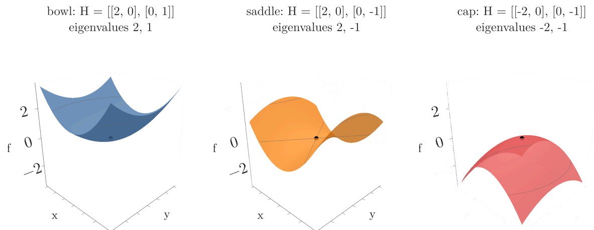
Figure 8: Three surfaces and the eigenvalues of their Hessians: both positive (bowl), opposite signs (saddle), both negative (cap)
