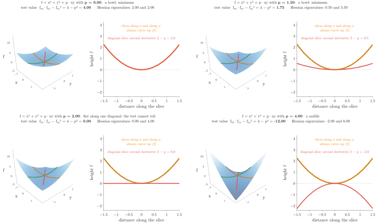
Figure 7: The surface f = x^2 + y^2 + pxy as p grows from 0 to 4. The slices along x and y (orange, green) never change; the diagonal slice (red) flattens at p = 2 and then bends down, so the bowl becomes a saddle. The title tracks the test value 4 - p^2 and the Hessian's eigenvalues 2 - p and 2 + p . Idea after Khan Academy, "Second partial derivative test"
