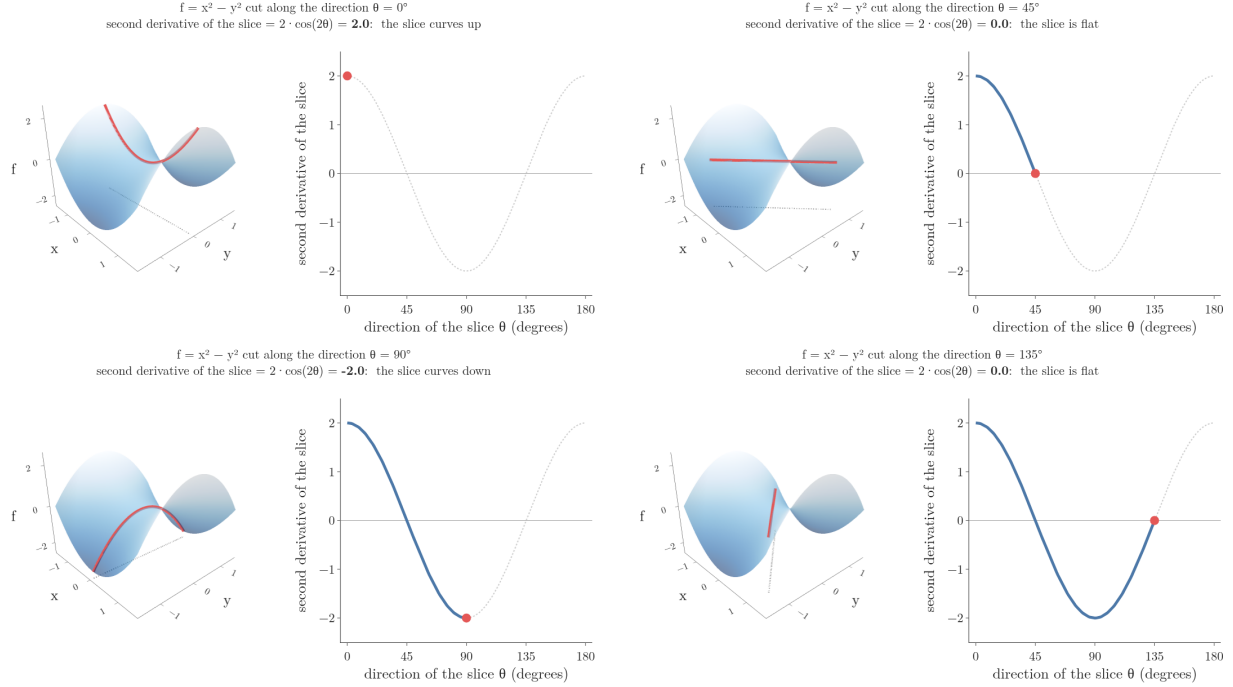
Figure 6: The saddle f = x^2 - y^2 cut by a vertical plane that turns from the x direction (angle 0) to the y direction (90 degrees). Left: the slice (red) on the surface. Right: the second derivative of the slice, 2 \cos 2\theta , traced against the angle: positive, zero, then negative. Idea after Khan Academy, “Saddle points”
