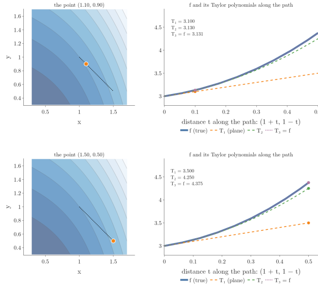
Figure 10: The Taylor polynomials of f(x, y) = x^3 + xy + y^2 around (1, 1) along the path to (1.5, 0.5) . Left: the moving point on the contour map of Figure 9. Right: f (thick blue) against T_1 , T_2 and T_3 ; T_3 equals f .
