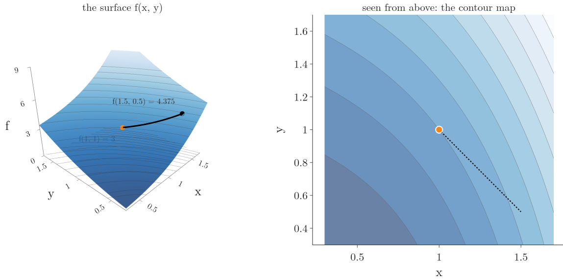
Figure 9: The surface f(x, y) = x^3 + xy + y^2 near (1, 1) (left), with its contour lines drawn on it and dropped to the floor, and the same surface seen from above as a contour map (right). Same colours, same square, same path from (1, 1) (orange) to (1.5, 0.5)
