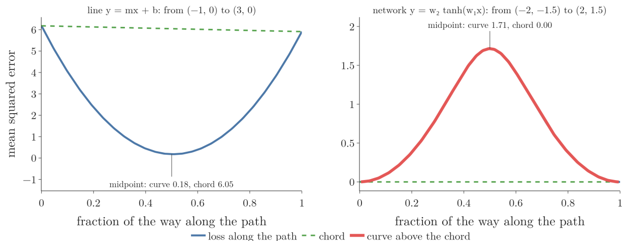
Figure 5: The chord test along a straight path in parameter space. Left: the line model, from (m, b) = (-1, 0) to (3, 0) ; the loss (blue) stays below the chord (dashed). Right: the tiny network, between its two minima (-2, -1.5) and (2, 1.5) ; the loss rises above the chord (red), to 1.71 at the midpoint.
