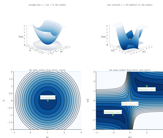
Figure 1: One dataset, two models. Top: the loss as a surface over the two parameters, with contour lines drawn on it and dropped to the floor. Bottom: the same surfaces seen from above, as contour maps. The loss of a straight line is one bowl (left); the loss of a tiny neural network has two separate minima with a ridge between them (right)
