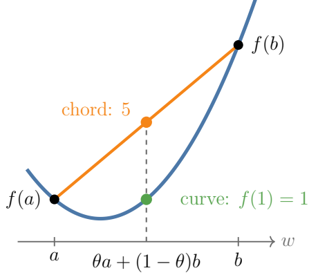
Figure 3: The chord test. Left: for w^2 , the curve at the midpoint (1) is below the chord (5): convex. Right: for g(w) = w^4 - 4w^2 + w , the curve at the midpoint (0) is above the chord (-3.94): non-convex
