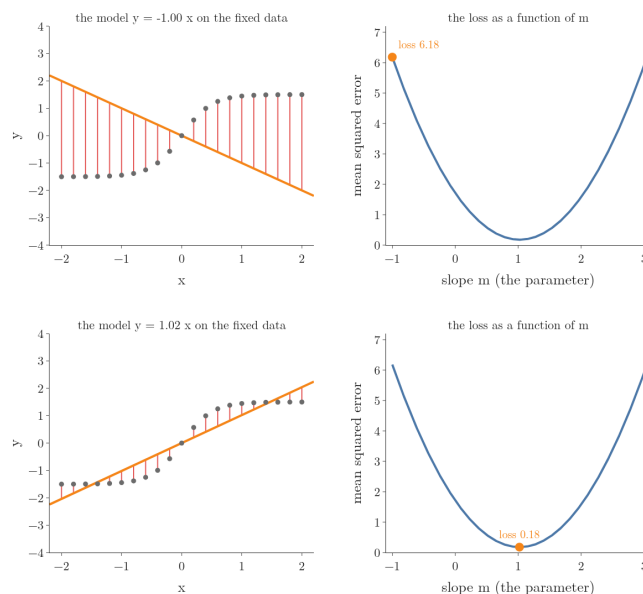
Figure 2: The loss as a function of one parameter. Left: the line y = mx on the fixed data, with its errors, as the slope m changes from -1 to 3 . Right: the mean squared error for each m ; the lowest point is m = 1.02 , loss 0.18 .
