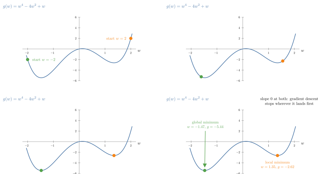
Figure 4: Gradient descent on g(w) = w^4 - 4w^2 + w with learning rate 0.02, started at w = -2 (green) and w = 2 (orange). Key frames: the two starts, after two steps, after 30 steps, and the two end points
