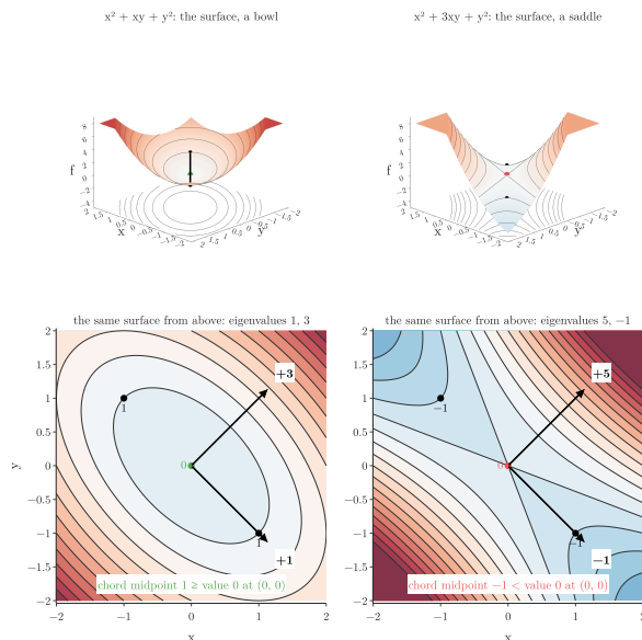
Figure 8: Top: the surfaces of the two quadratics (the black segment is the chord between (1, -1) and (-1, 1) ). Bottom: the same surfaces seen from above, as contour maps. Arrows: the Hessian's eigenvector directions, labelled with their eigenvalues. Left: both positive, closed ellipses, a bowl. Right: one negative, a saddle; the chord between (1, -1) and (-1, 1) sits at -1 , below the value 0 at the midpoint
