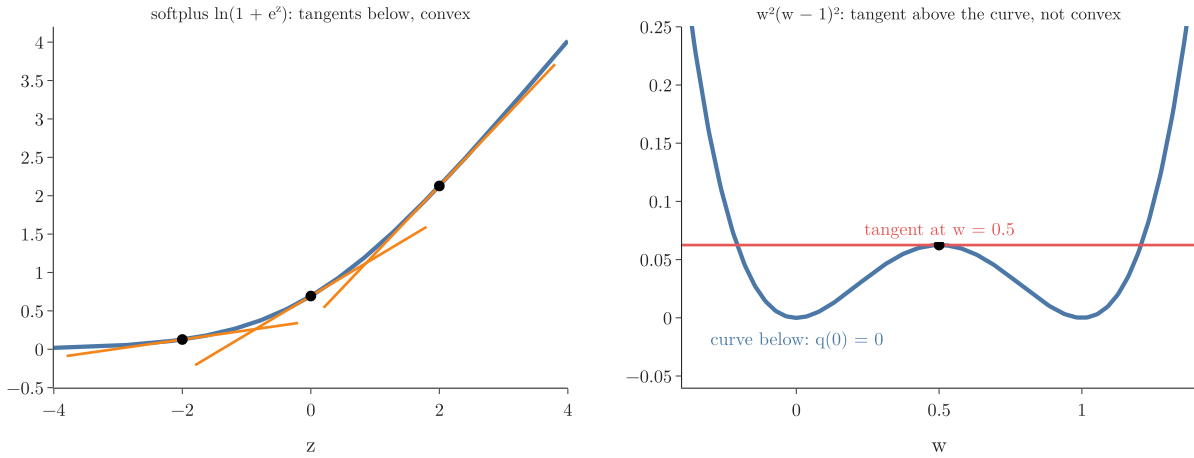
Figure 7: The first-order test. Left: every tangent of softplus lies below the curve, so it is convex. Right: the tangent of w^2(w-1)^2 at w = 0.5 lies above the curve near 0 and 1, so it is not convex
