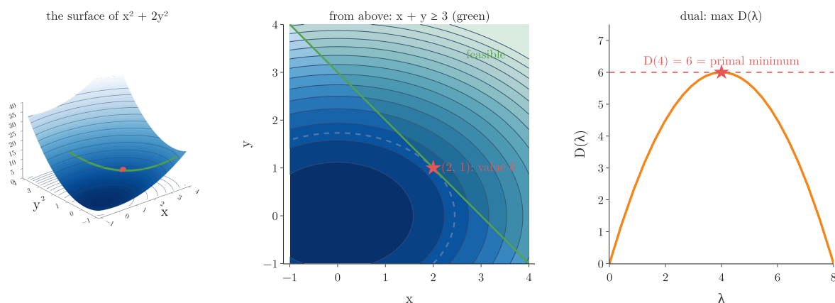
Figure 10: Left: the surface of x^2 + 2y^2 (a bowl) with the line x + y = 3 lifted onto it (green) and the lowest allowed point (red). Middle: the same surface from above, as contours of x^2 + 2y^2 , and the feasible half-plane x + y \geq 3 (green); the lowest feasible point is (2, 1) , on the contour of value 6 (dashed). Right: the dual function D(\lambda) = 3\lambda - 3\lambda^2/8 peaks at \lambda = 4 with the same value 6
