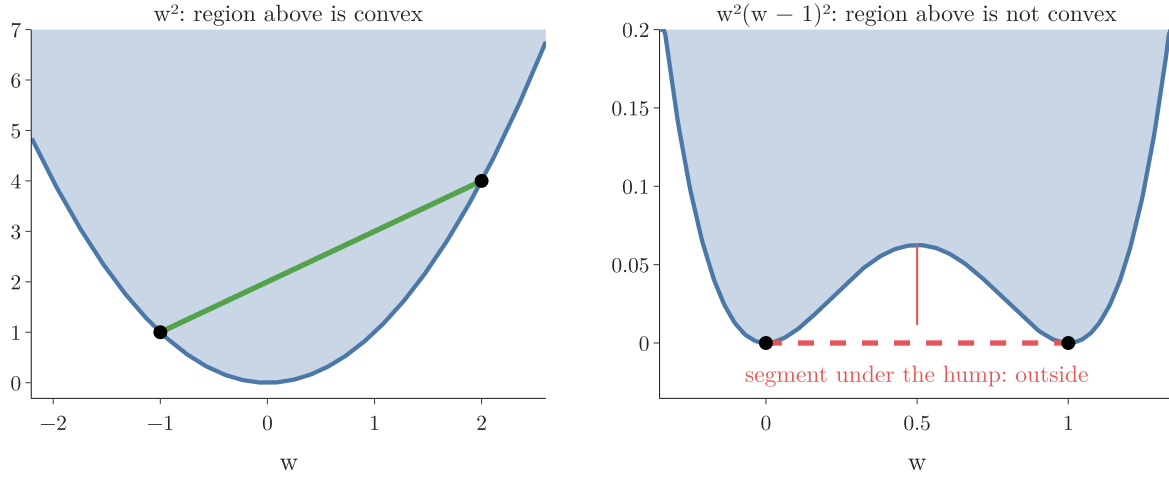
Figure 5: The epigraph, shaded: the region on and above each graph. Left: for w^2 , the segment between two points of the region (green) stays inside, so the region is a convex set. Right: for w^2(w-1)^2 , the segment from (0, 0) to (1, 0) runs under the hump, outside the region (red dashed)
