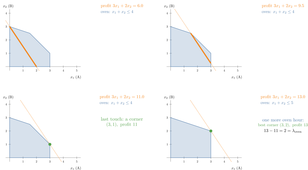
Figure 3: The profit line 3x_1 + 2x_2 = p slides outward; its feasible part (thick orange) shrinks until it touches only the corner (3, 1) at p = 11 . Then one more oven hour moves the best corner to (3, 2) , profit 13. Key frames: p = 6, 9.5, 11 , and oven limit 5
