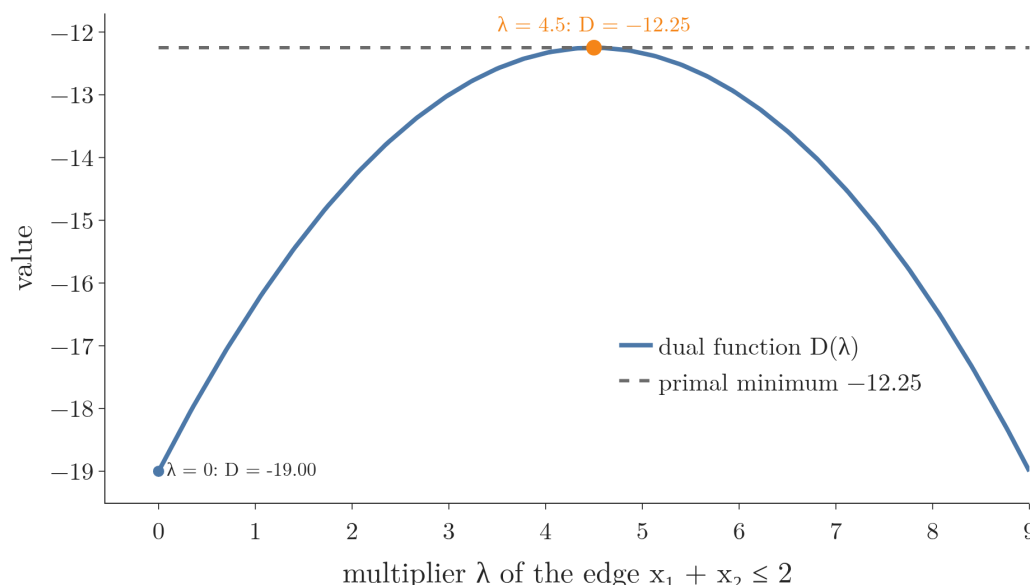
Figure 10: The dual function of the quadratic program along the edge multiplier \lambda (the other two multipliers at 0): a concave curve below the primal minimum -12.25 (dashed), touching it at \lambda = 4.5 .
