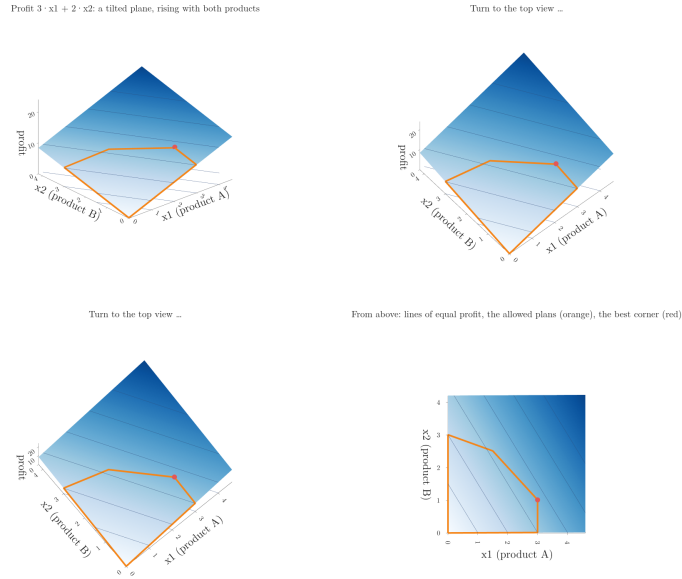
Figure 2: The profit 3x_1 + 2x_2 as a surface over the plans: a tilted plane. The allowed plans (orange) lifted onto it, and the best corner (red). Last frame: the same plane from above, as parallel lines of equal profit
