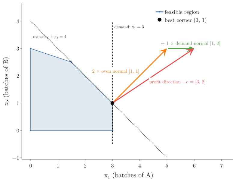
Figure 5: The dual condition at the best corner (3, 1) . The profit direction -c = [3, 2] (red) equals 2 times the oven normal [1, 1] (orange) plus 1 times the demand normal [1, 0] (green): non-negative weights, the multipliers 2 and 1.
