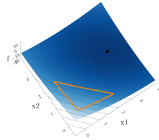
Figure 7: The bowl f(x_1, x_2) of the quadratic program as a surface, with the triangle lifted onto it (orange), its bottom (3, 2) (black) and the constrained minimum (1.5, 0.5) (green). The camera tilts to the top view, the contour map of Figure 8
