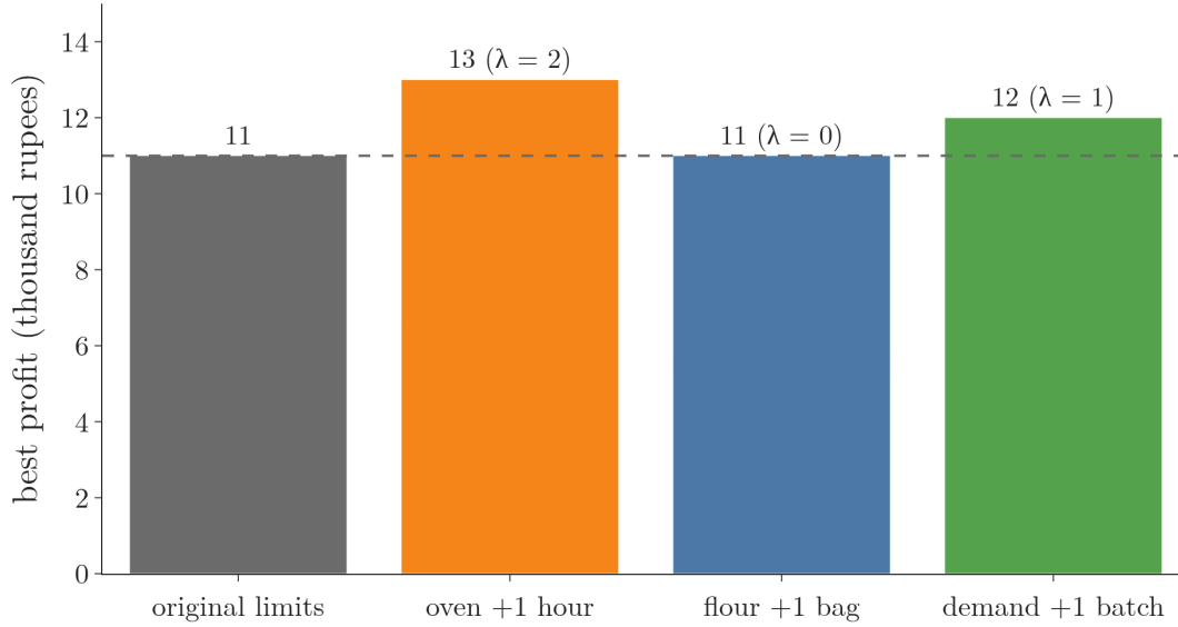
Figure 6: The best profit re-solved with one more unit of each resource. Oven: 13, up by 2. Flour: 11, unchanged. Demand: 12, up by 1. The rises are the multipliers.
