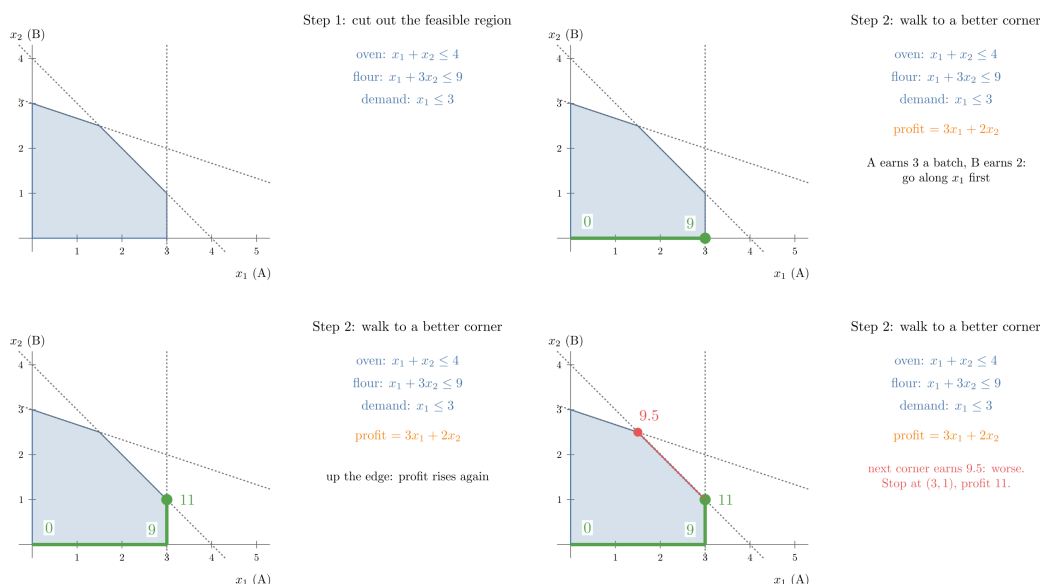
Figure 4: The workshop region cut out one constraint at a time (oven, flour, demand), then the walk from vertex to vertex: profit 0, 9, 11. The next vertex earns 9.5 (red), so the walk stops at (3, 1) . Idea after StatQuest, “Optimization with Linear Programming (and the Simplex Algorithm), Main Ideas!!!”; our own problem
