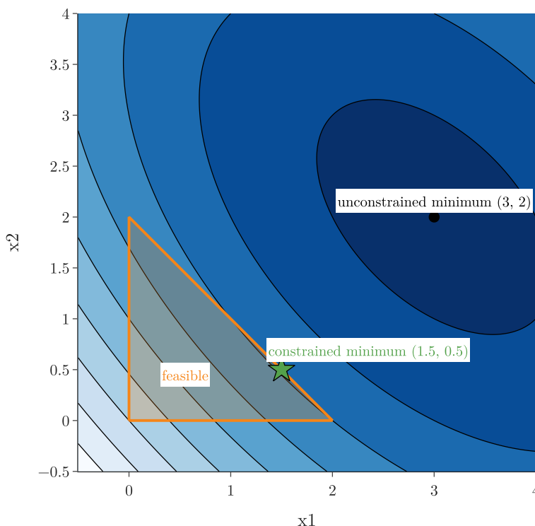
Figure 8: A quadratic program: the elliptical contours of a bowl with its unconstrained minimum at (3, 2) , and the triangular feasible region (orange). The constrained minimum (star) lies on the edge x_1 + x_2 = 2
