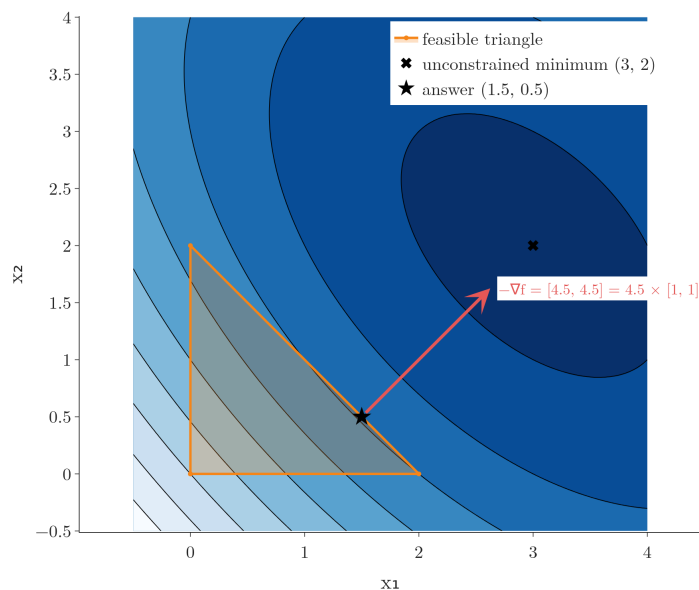
Figure 9: The quadratic program at its answer (1.5, 0.5) (star). The downhill direction -\nabla f = [4.5, 4.5] (red) is 4.5 times the normal of the active edge x_1 + x_2 = 2 ; the unconstrained minimum (3, 2) lies outside the triangle.
