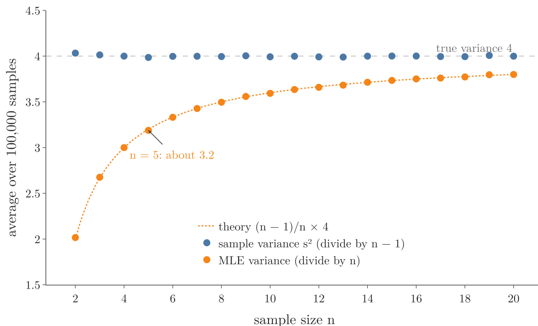
Figure 8: Averages over 100,000 simulated samples of each size n from a population with variance 4. Blue: the sample variance, about 4 for every n . Orange: the MLE variance, on the curve (n - 1)/n \times 4 , about 3.2 at n = 5 and closing on 4 as n grows
