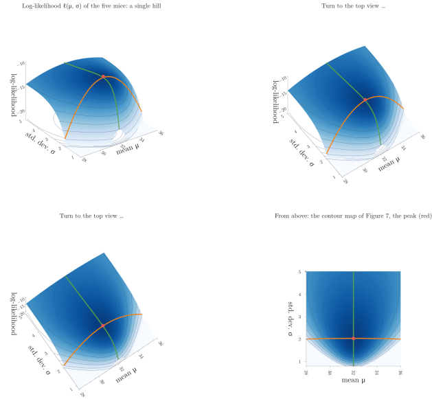
Figure 6: The log-likelihood of the five mouse weights as a surface over the mean and the standard deviation: one hill with its top at (32, 2) . The orange and green curves are the two one-parameter searches. The camera then tilts to the top view, the contour map of Figure 7
