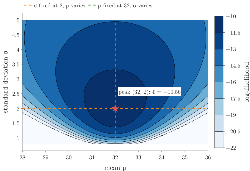
Figure 7: Contour map of the normal log-likelihood of the five mouse weights over the mean and the standard deviation, with a single peak at (32, 2) (Figure 6 from above)
