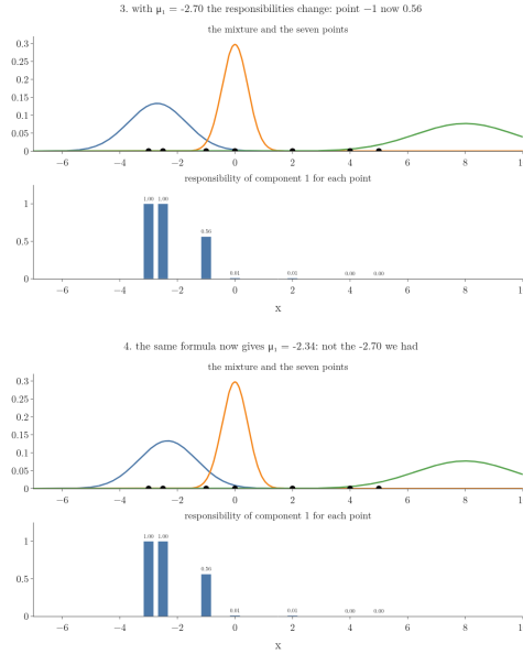
Figure 9: The circular dependence on the seven points. 1: the starting mixture. 2: the slope-zero formula moves \mu_1 from -4 to -2.70 . 3: with the new \mu_1 the responsibilities change; point -1 now belongs 0.56 to component 1. 4: the same formula now gives -2.34 .
