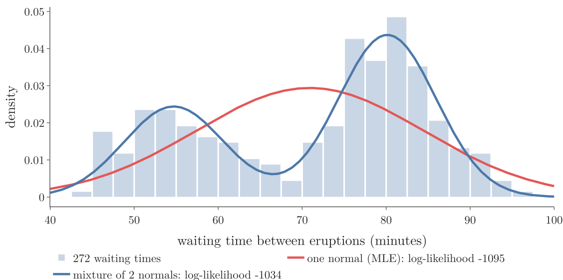
Figure 1: Waiting times between Old Faithful eruptions: the best single normal (red) and a fitted mixture of two normals (blue)
