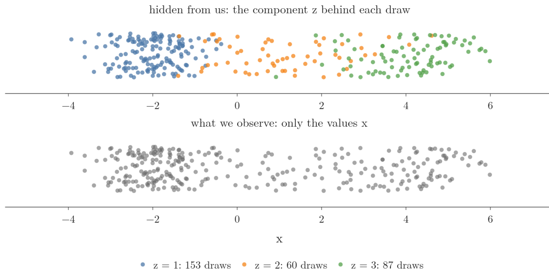
Figure 5: 300 draws from the mixture of Figure 6. Top: coloured by the component z that produced each draw, which the sampler knows but we never see. Bottom: the same draws as we observe them, with z lost.
