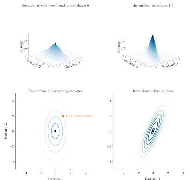
Figure 7: Two-dimensional normal components with variances 1 and 4. Top: the density as a surface (a hill). Bottom: the same hill seen from above, as a contour map. Left: no covariance, ellipses along the axes; the example point (1, 2) has density 0.0293. Right: covariance 1.6, tilted ellipses.
