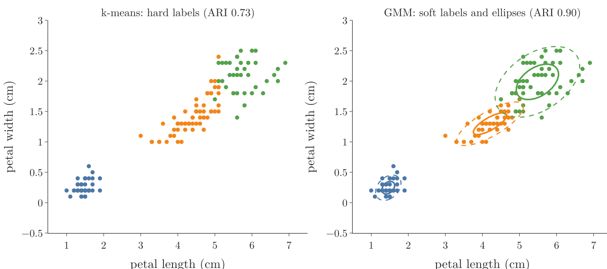
Figure 11: Iris, petal length against petal width. Left: k-means labels. Right: GMM with full covariance matrices; colours mix by responsibility, ellipses show 1 and 2 standard deviations
