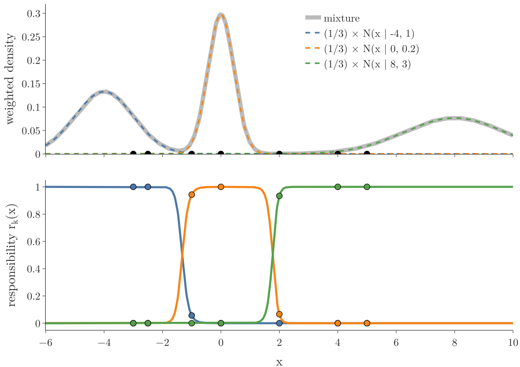
Figure 8: Top: the starting mixture of the book’s example and its seven points. Bottom: the responsibility of each component across x , with the seven points marked
