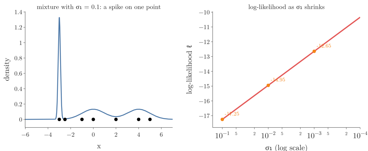
Figure 10: Collapse of maximum likelihood on the seven points. Left: the mixture with component 1 on the point -3 and \sigma_1 = 0.1 , a spike on one point. Right: the log-likelihood as \sigma_1 shrinks from 0.1 to 0.0001; it rises in a straight line on the log scale, without limit.
