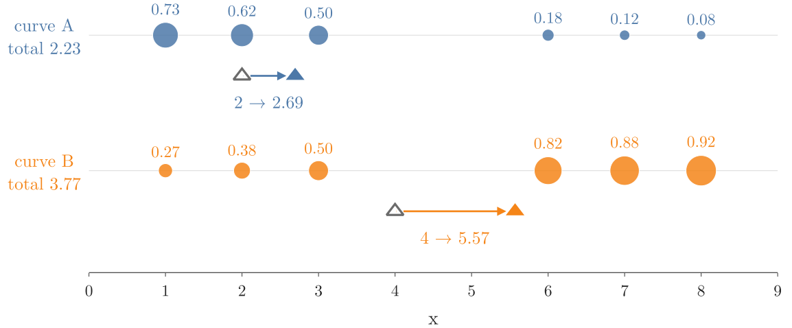
Figure 3: The update on the six points. Row A and row B: each point is as large as its share of that curve (label). Each centre moves from its start (hollow triangle) to the share-weighted average (filled triangle)
