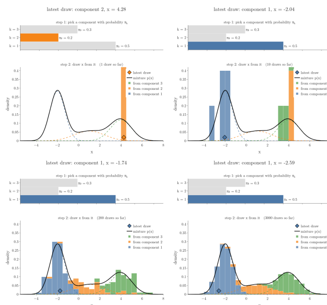
Figure 4: Sampling from a mixture in two steps. Top: pick one of three normal curves with probabilities 0.5, 0.2 and 0.3. Bottom: draw a value from the picked curve. As the draws pile up, their histogram takes the shape of the mixture density (black)
