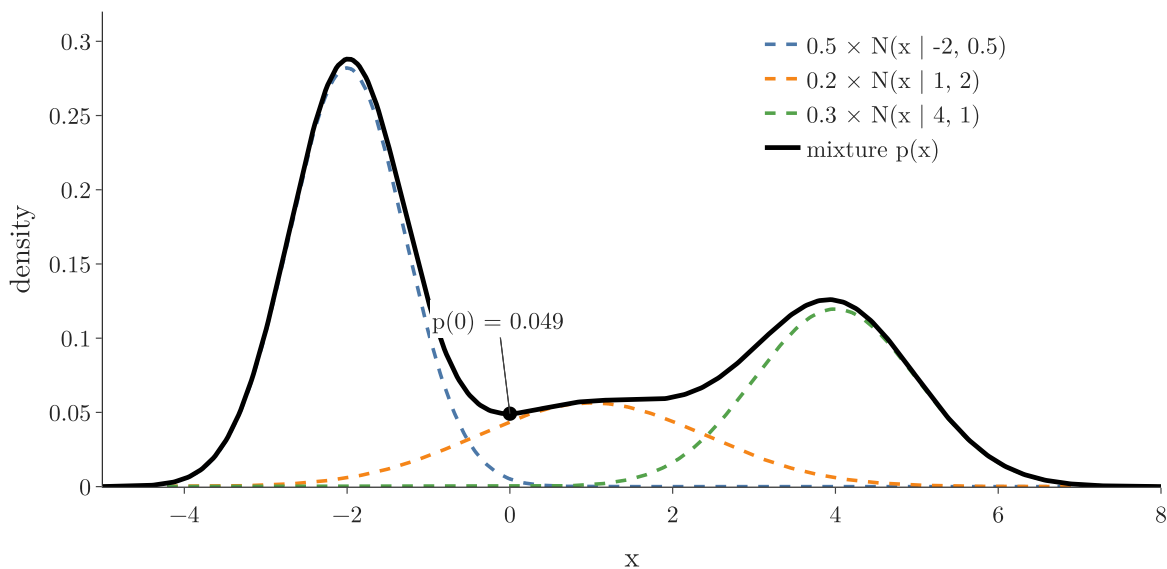
Figure 6: The mixture 0.5 N(-2, 0.5) + 0.2 N(1, 2) + 0.3 N(4, 1) : weighted components (dashed) and the mixture density (black)
