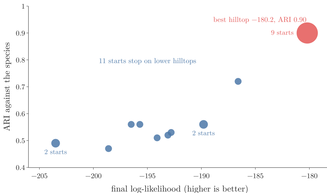
Figure 7: EM from 20 random starts on the Iris flowers. Each dot is one final answer: its log-likelihood (right is better) and its match with the species (ARI); dot size grows with the number of starts that ended there. Red: the best hilltop, reached by 9 starts
