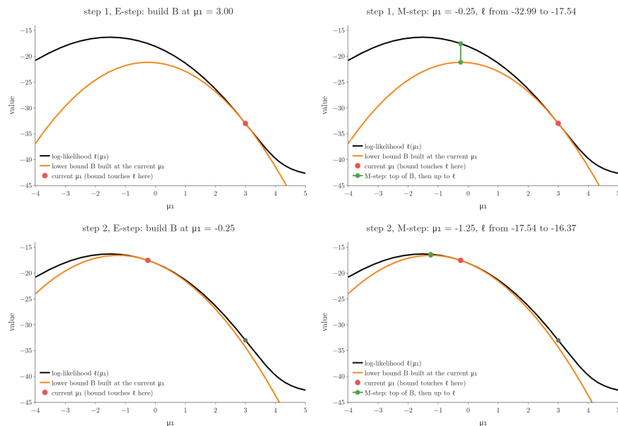
Figure 6: EM as climbing lower bounds. Black: the log-likelihood of \mu_1 . Orange: the bound built by the E-step, touching at the current \mu_1 . Green: the M-step jumps to the bound's top; the log-likelihood rises at least as much
