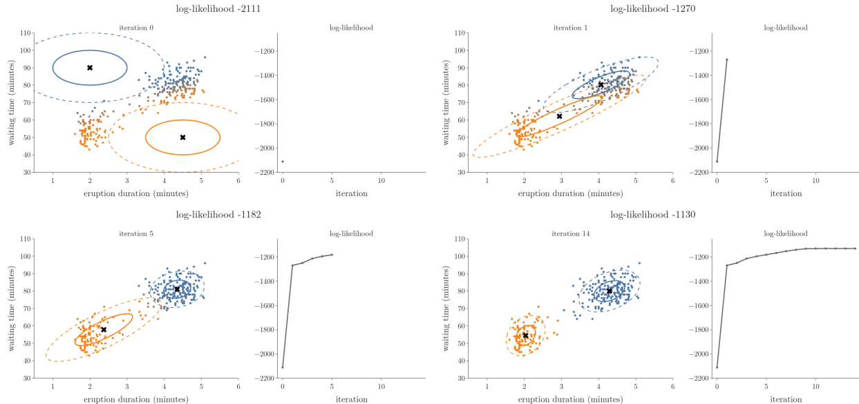
Figure 5: EM on the 272 eruptions of the Old Faithful geyser from a poor start. Left: each eruption’s colour mixes the two component colours by its responsibilities; ellipses show 1 and 2 standard deviations. Right: the log-likelihood after each iteration only goes up
