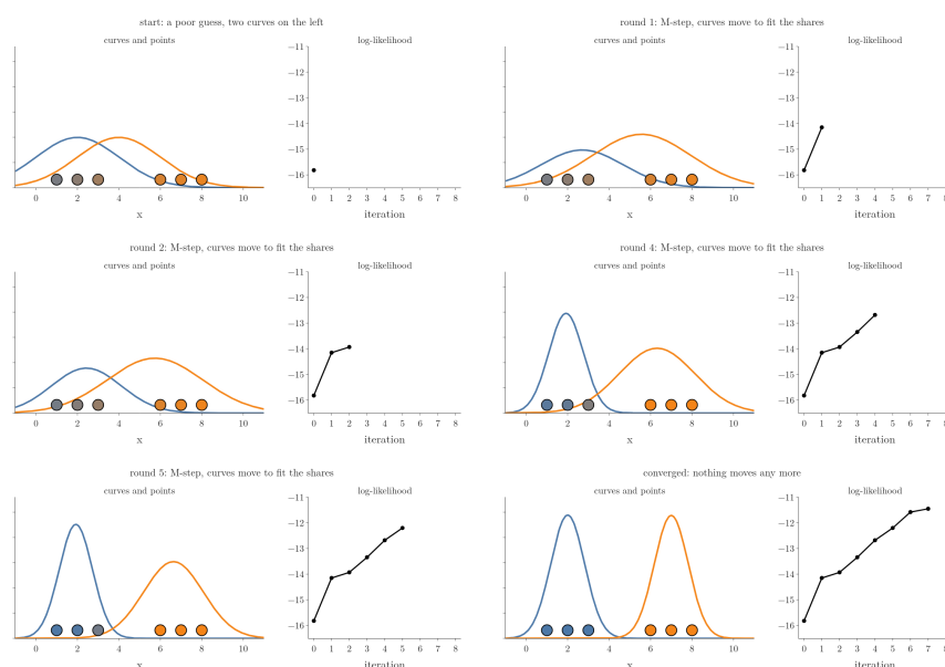
Figure 1: EM on six points, from a poor start of two curves on the left. Each round has two frames. E-step: every point is coloured by its shares of curve A (blue) and curve B (orange). M-step: the curves move and change width to fit the shares. Right: the log-likelihood after each round only goes up
