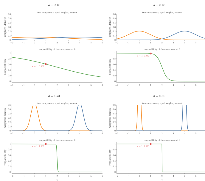
Figure 8: Two components with equal weights at 0 and 4 while their common \sigma shrinks from 3 to 0.1. Top: the two weighted normal curves. Bottom: the responsibility of the component at 0 across x ; the red dot is the observation at x = 1 . The curve sharpens into a step at the midpoint 2
