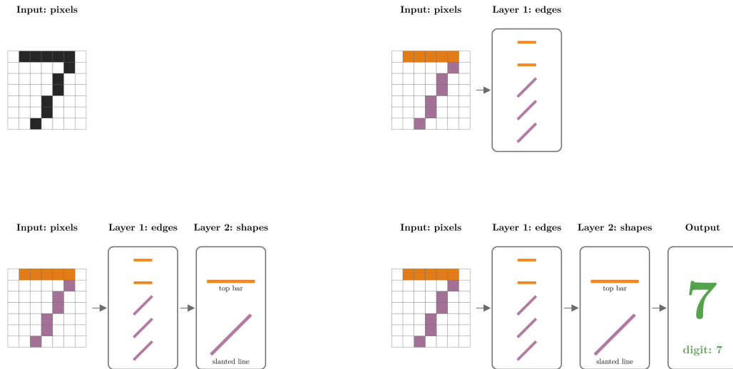
Figure 9: Layers of a neural network recognising a handwritten 7
