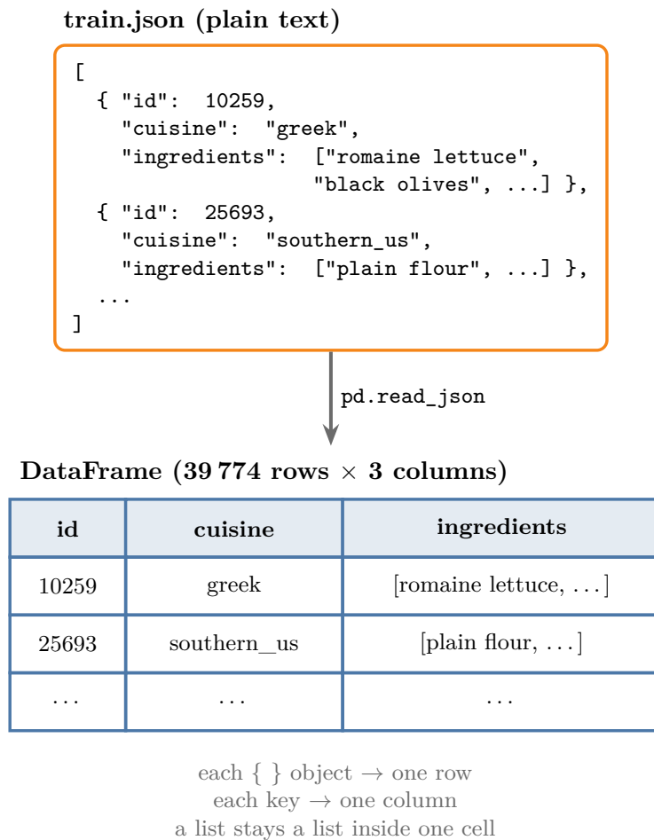
Figure 3: From JSON text to a DataFrame
