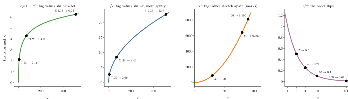
Figure 9: The four transforms of this section as curves, with the worked examples on them: \log(1 + x) and the square root for the fares 7.25, 71.28 and 512.33; the square for the marks 30, 80 and 90; 1/x for 2, 4, 10 and 100 (log x axis).
