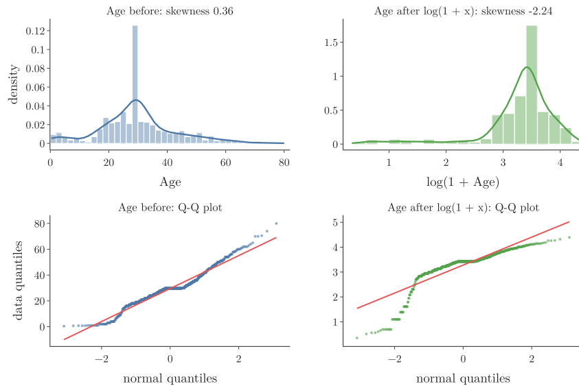
Figure 12: Age before (blue) and after (green) the log transform: density plot and Q-Q plot
