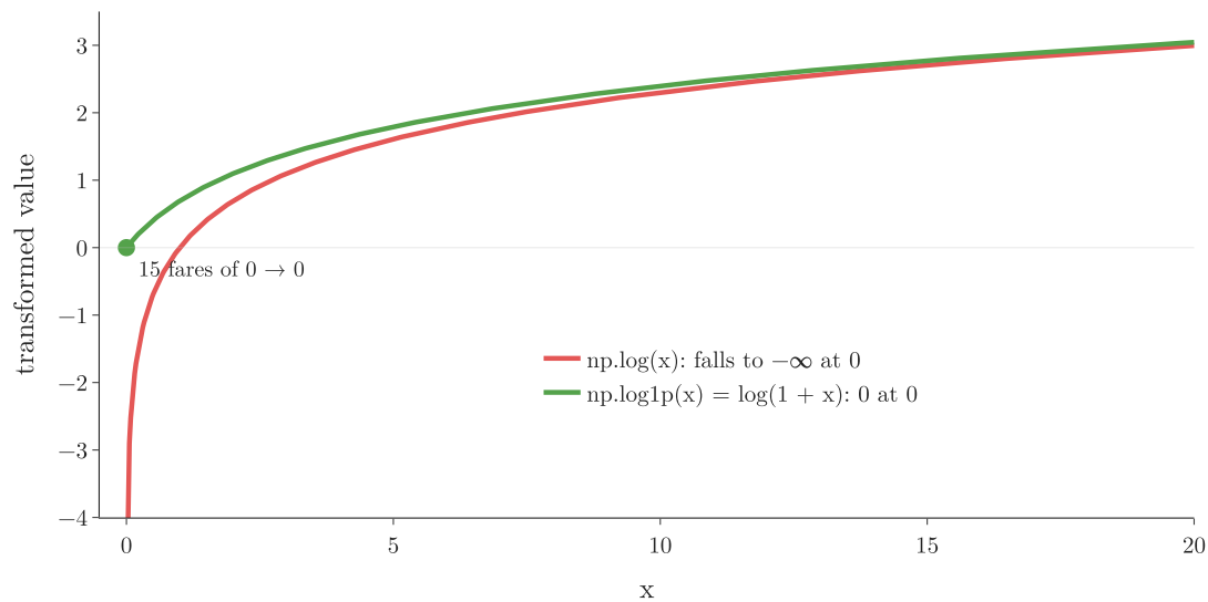
Figure 8: np.log(x) (red) and np.log1p(x) (green). At 0 the plain log has no value; \log(1 + x) maps the 15 zero fares to 0. For large x the two are almost equal.
