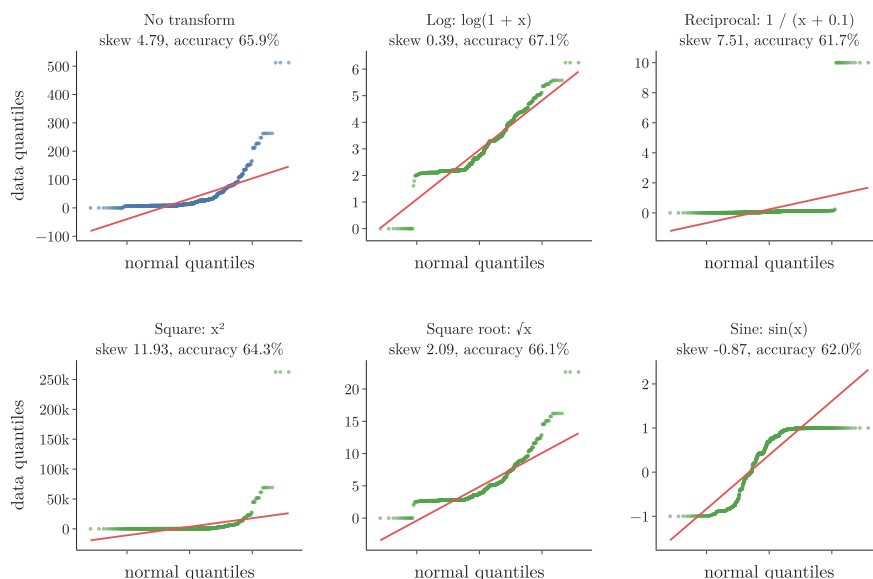
Figure 13: Fare after each transform: Q-Q plot, skewness and cross-validated accuracy of logistic regression
