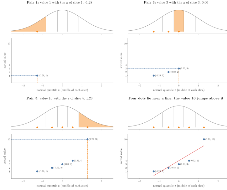
Figure 4: A Q-Q plot built one pair at a time for the values 1, 2, 3, 4 and 10. Top: the normal curve in five equal-probability slices, with the z -value of each. Bottom: each sorted value against its z -value. Construction after StatQuest, “Quantile-Quantile Plots (QQ plots), Clearly Explained!!!”.
