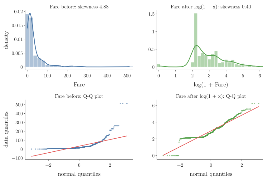
Figure 10: Fare before (blue) and after (green) the log transform: density plot and Q-Q plot
