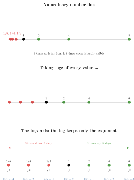
Figure 7: The values 1/8 to 8 sliding from an ordinary number line to a \log_2 axis. The log keeps only the exponent, so each doubling or halving becomes one equal step. Idea after StatQuest, “Logs (logarithms), Clearly Explained!!!”.
