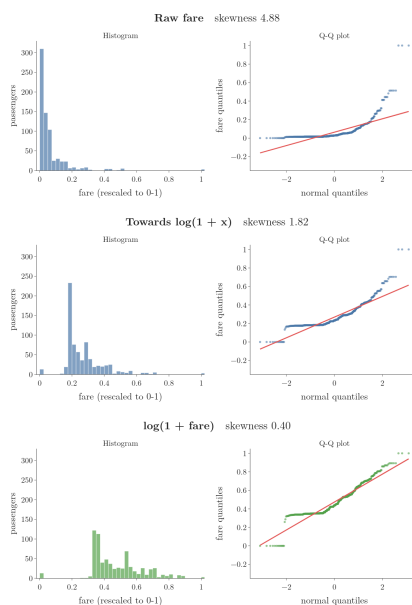
Figure 11: The training fares sliding from raw values to \log(1 + x) , with the axis rescaled to 0-1 in every frame: histogram (left) and Q-Q plot (right). The skewness falls from 4.88 to 0.40.
