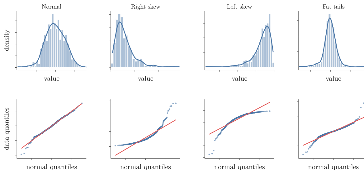
Figure 5: Four shapes of data (top) and their Q-Q plots (bottom)
