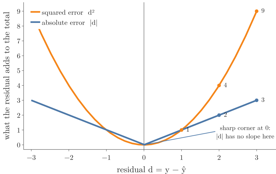
Figure 5: What one residual d adds to the total: d squared (orange) against the absolute value of d (blue). Residuals of 1, 2 and 3 add 1, 4 and 9 when squared.
