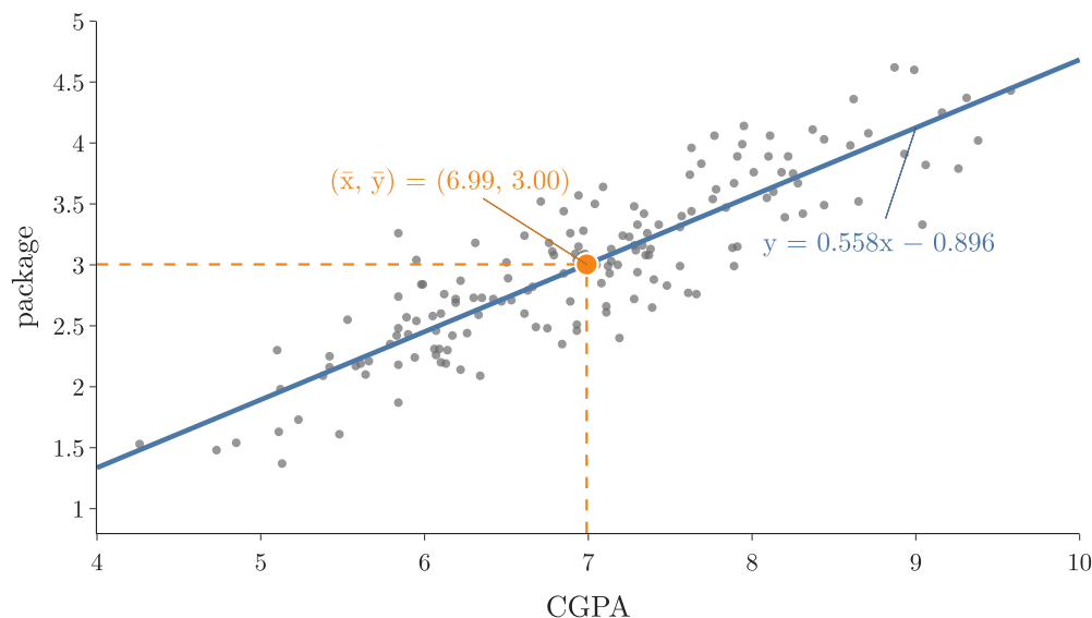
Figure 10: The OLS line on the 160 training students passes through the point of means (6.99, 3.00)
