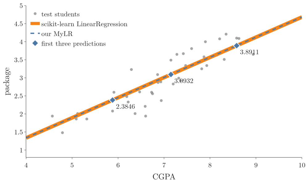
Figure 12: On the 40 test students, the line of our MyLR class (dashed blue) lies on top of scikit-learn's LinearRegression line (orange). Diamonds: the first three test predictions, 3.8911, 3.0932 and 2.3846.
