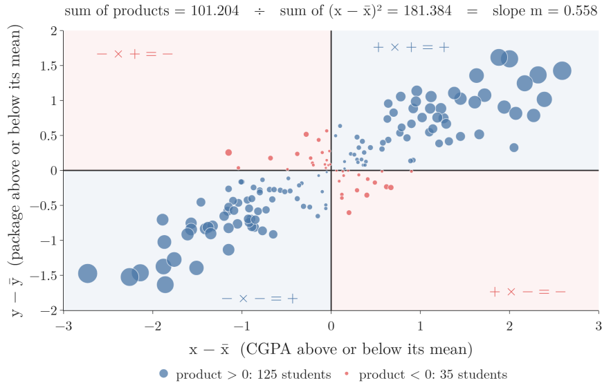
Figure 9: The 160 training students with the axes moved to the point of means. Each dot's size is the size of its product; blue products are positive, red negative. Sum of products 101.204, divided by the sum of squared CGPA deviations 181.384, gives m = 0.558 .
