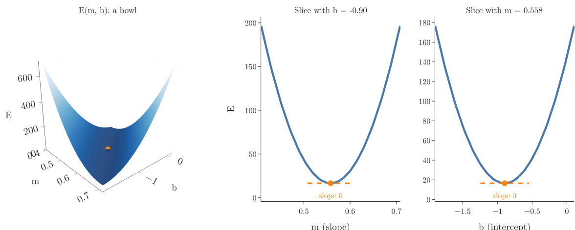
Figure 7: The error function: a bowl with the best line at the bottom
