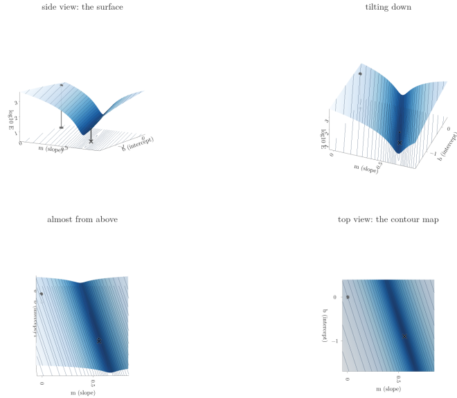
Figure 1: The error surface E(m, b) on the 160 training students, seen from the side and then tilted to the top view. Height is \log_{10} E . Black cross: the best line ( m = 0.558 , b = -0.896 ). Grey square: the start m = 0 , b = 0 . The final frame is the contour map used in Figure 2 and Figure 6.
