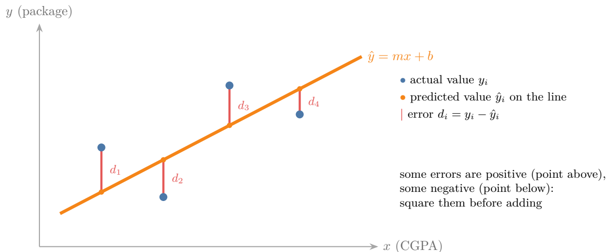
Figure 3: The error at each point is the vertical gap to the line
