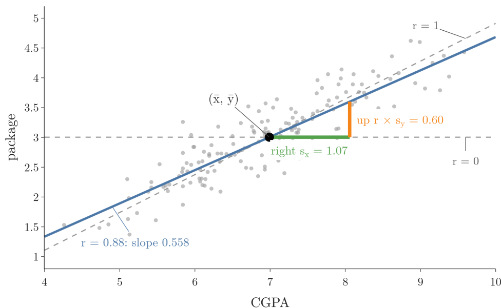
Figure 11: The best-fit line drawn from the point of means: right by s_x , up by r \times s_y . Dashed: the line if r were 1 (up a full s_y ) and if r were 0 (flat at the average package). Idea after Khan Academy, “Calculating the equation of a regression line”.
