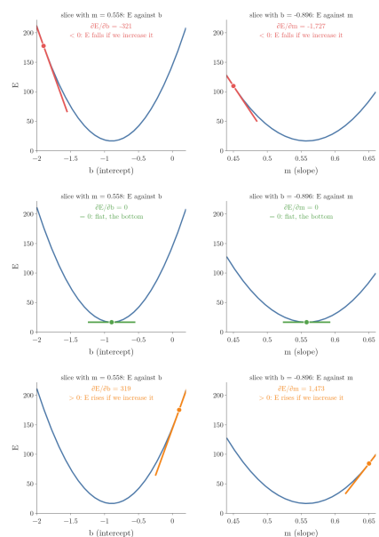
Figure 8: A tangent line slides along each slice of the bowl. Its slope is the partial derivative: negative (red) before the bottom, 0 (green) at m = 0.558 and b = -0.896 , positive (orange) after.
