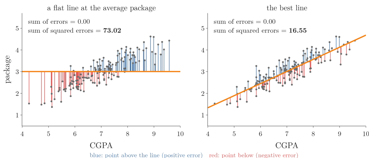
Figure 4: Two lines on the 160 training students. Blue sticks: positive residuals; red sticks: negative ones. For both lines the residuals add up to 0, but the sums of squared residuals are 73.02 for the flat line and 16.55 for the best line.
