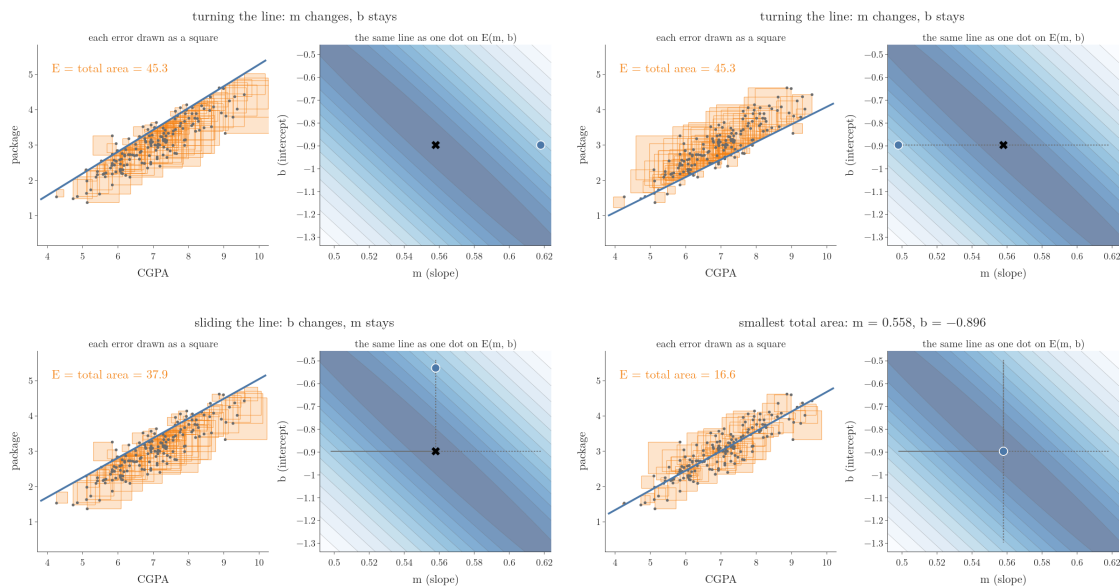
Figure 6: Turning and sliding a line through the 160 training students. Left: the squared errors as squares, with total area E . Right: the same line as a dot on the contour map of E(m, b) ; the black cross marks the smallest E .
