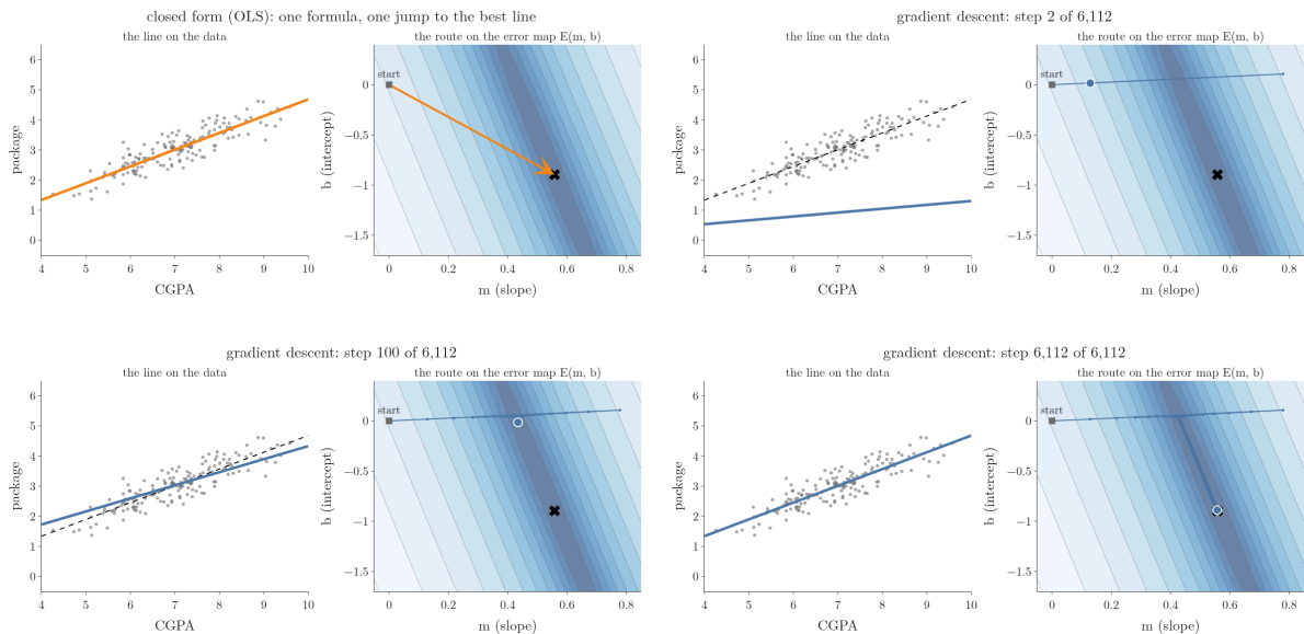
Figure 2: Two routes to the best line on the 160 training students. Orange: OLS computes m = 0.558 , b = -0.896 in one step. Blue: gradient descent from (0, 0) , learning rate 0.018, reaches the same line after 6,112 small steps. Left: the line on the data; right: the route on the error map.
