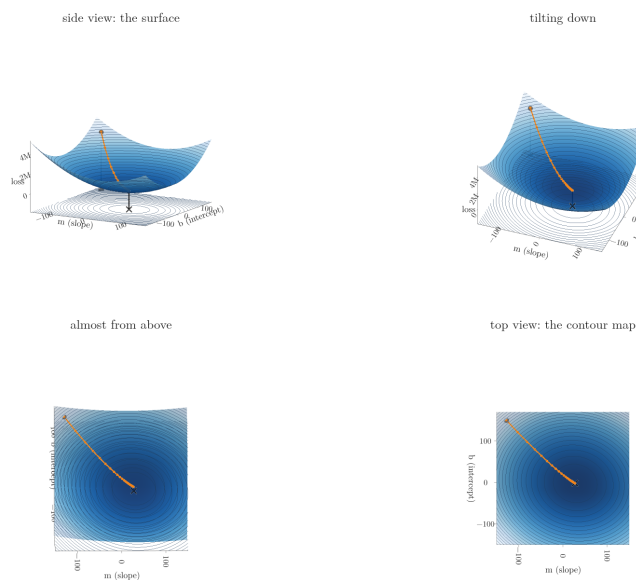
Figure 6: The loss surface L(m, b) of the 100 points, seen from the side and tilted to the top view, with the 30-epoch descent path in orange. The final frame is the contour map of Figure 7.
