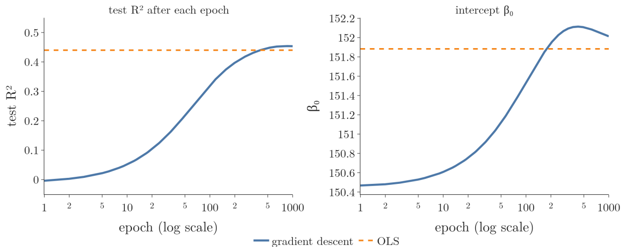
Figure 4: What the GDRegressor code produces on the diabetes data, learning rate 0.5. Left: test R^2 after each epoch against the OLS value. Right: the intercept against the OLS intercept. Both axes of epochs use a log scale.
