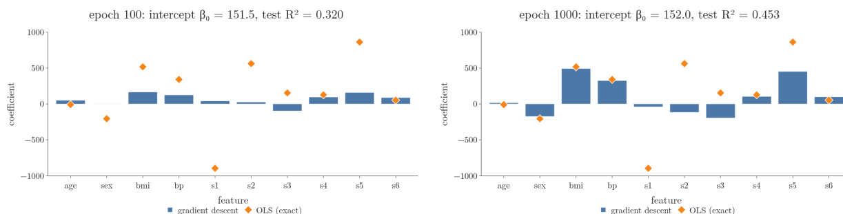
Figure 2: Batch gradient descent on the diabetes data (Section 4), epoch by epoch. Bars: the 10 coefficients, all updated at every step; diamonds: the exact OLS values. The title gives the intercept and the test R^2 .
