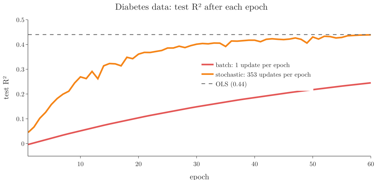
Figure 4: Test R^2 after each epoch: batch vs stochastic
