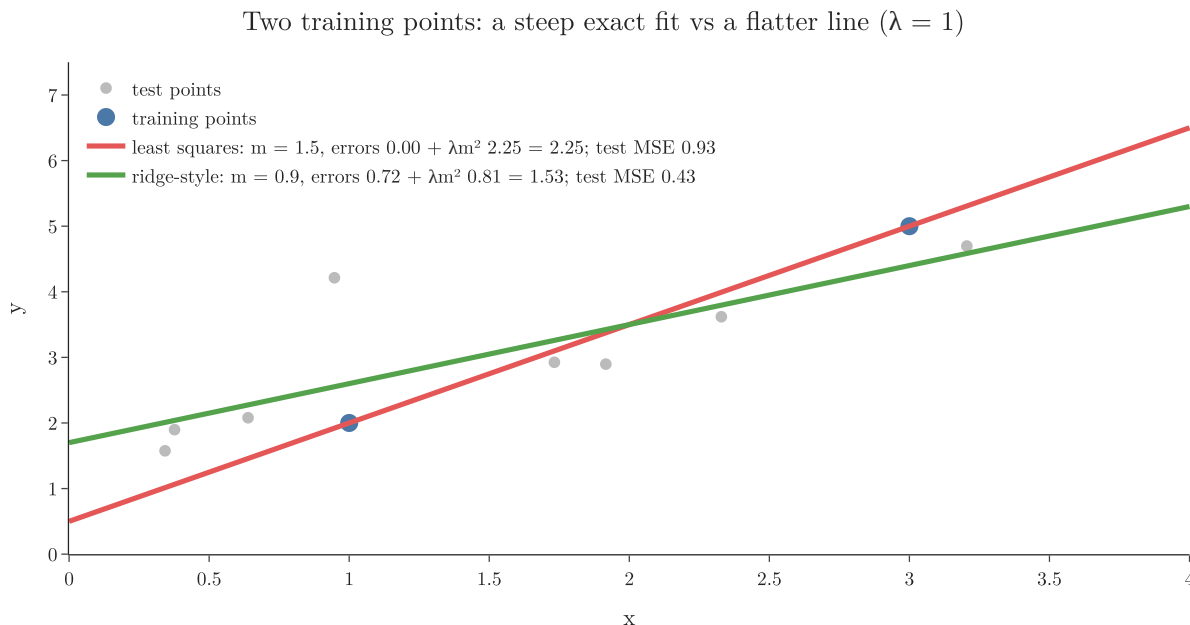
Figure 3: Two training points: the exact fit vs a flatter line
