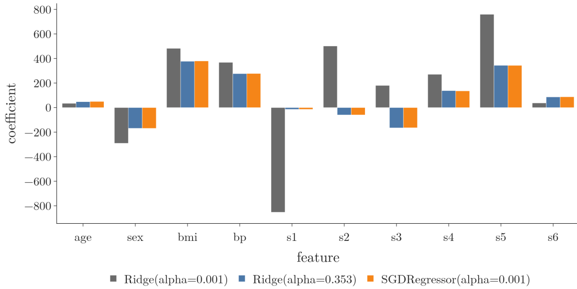
Figure 8: Coefficients on the diabetes training data (353 observations): Ridge with alpha 0.001 (grey) and 0.353 (blue), and SGDRegressor with alpha 0.001 run for 50,000 epochs (orange). The orange bars match the blue ones.
