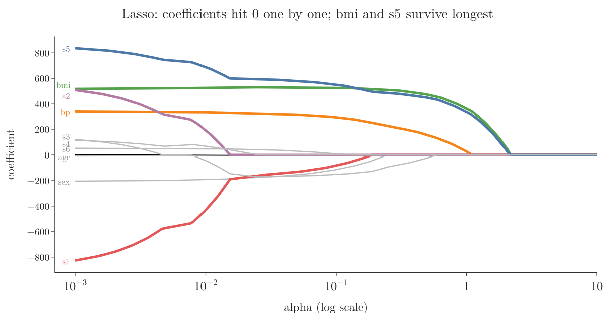
Figure 5: Lasso coefficient paths on the diabetes data
