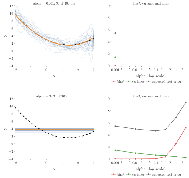
Figure 6: Bias and variance of Lasso on a degree-16 polynomial. Left: 30 of the 200 fitted curves (blue), their average (orange) and the true curve (dashed) for each alpha. Right: \text{bias}^2 , variance and expected test error, built up alpha by alpha; the error is lowest at alpha 0.1.
