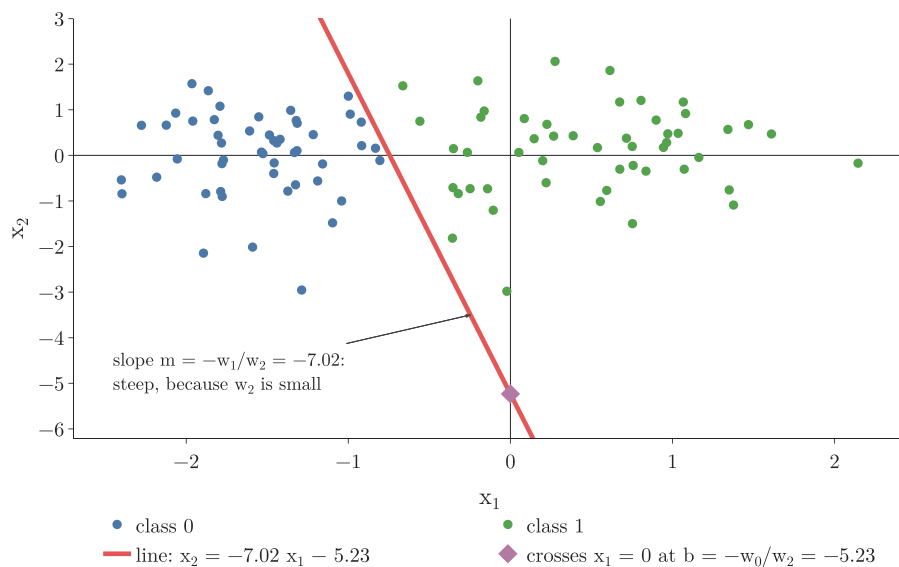
Figure 2: The final weights (1.00, 1.34, 0.19) drawn as the line x_2 = -7.02 x_1 - 5.23 . The diamond marks the intercept b = -w_0/w_2 ; the slope -w_1/w_2 is steep because w_2 is small.
