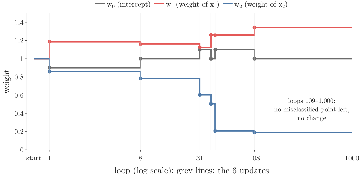
Figure 1: The weights w_0 , w_1 and w_2 after every loop of the seed-0 run (log scale for the loop number). They change only at loops 1, 8, 31, 40, 44 and 108, when the picked point was misclassified; loops 109 to 1,000 change nothing.
