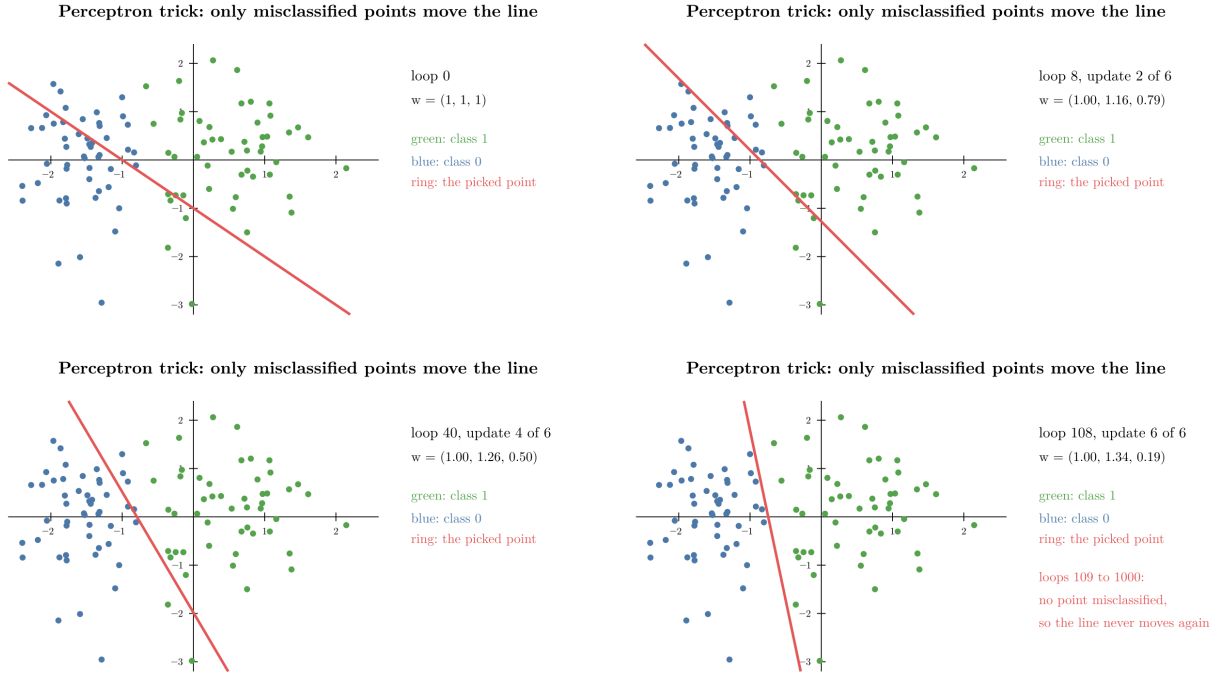
Figure 3: The perceptron trick on 100 points: the decision boundary after 0, 2, 4 and 6 updates
