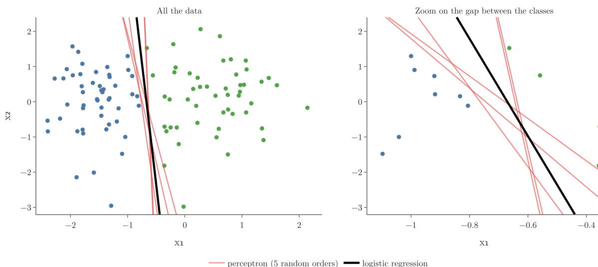
Figure 4: Five perceptron decision boundaries and the logistic regression boundary, with a zoom on the gap
