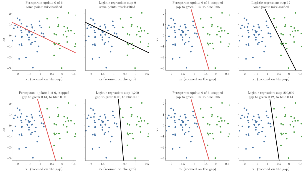
Figure 5: The perceptron trick (left, seed 0) and logistic regression trained by gradient descent (right) on the same 100 points, zoomed on the gap between the classes. The perceptron’s decision boundary stops after its 6th update, 0.06 from the nearest blue point. The logistic regression boundary keeps moving after every point is already on its correct side, and ends near the middle of the gap (0.12 and 0.14)
