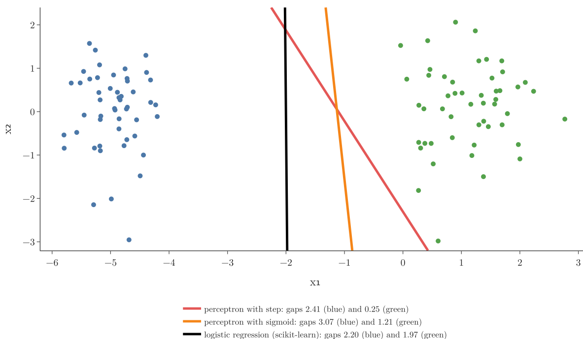
Figure 8: Step perceptron, sigmoid perceptron and logistic regression
