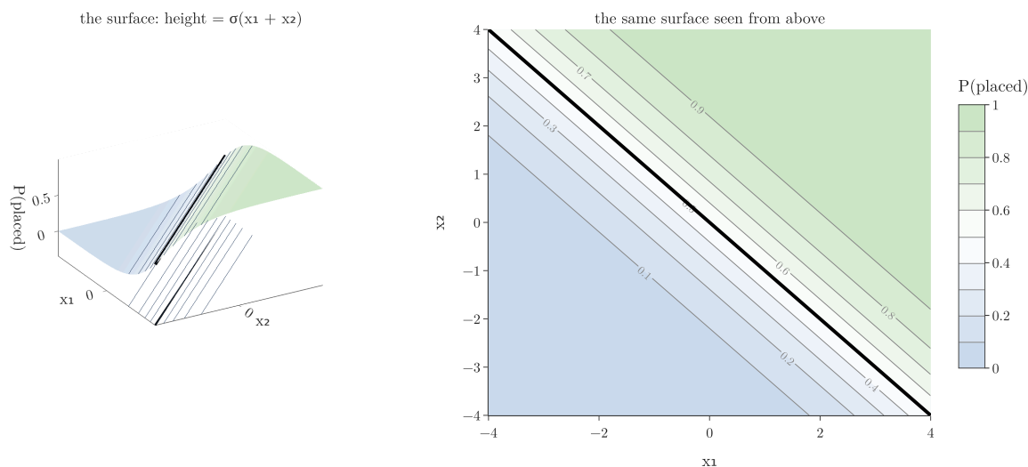
Figure 4: \sigma(w \cdot x) as the probability of being placed: the surface (left) and the same surface seen from above (right). The black line is \sigma = 0.5
