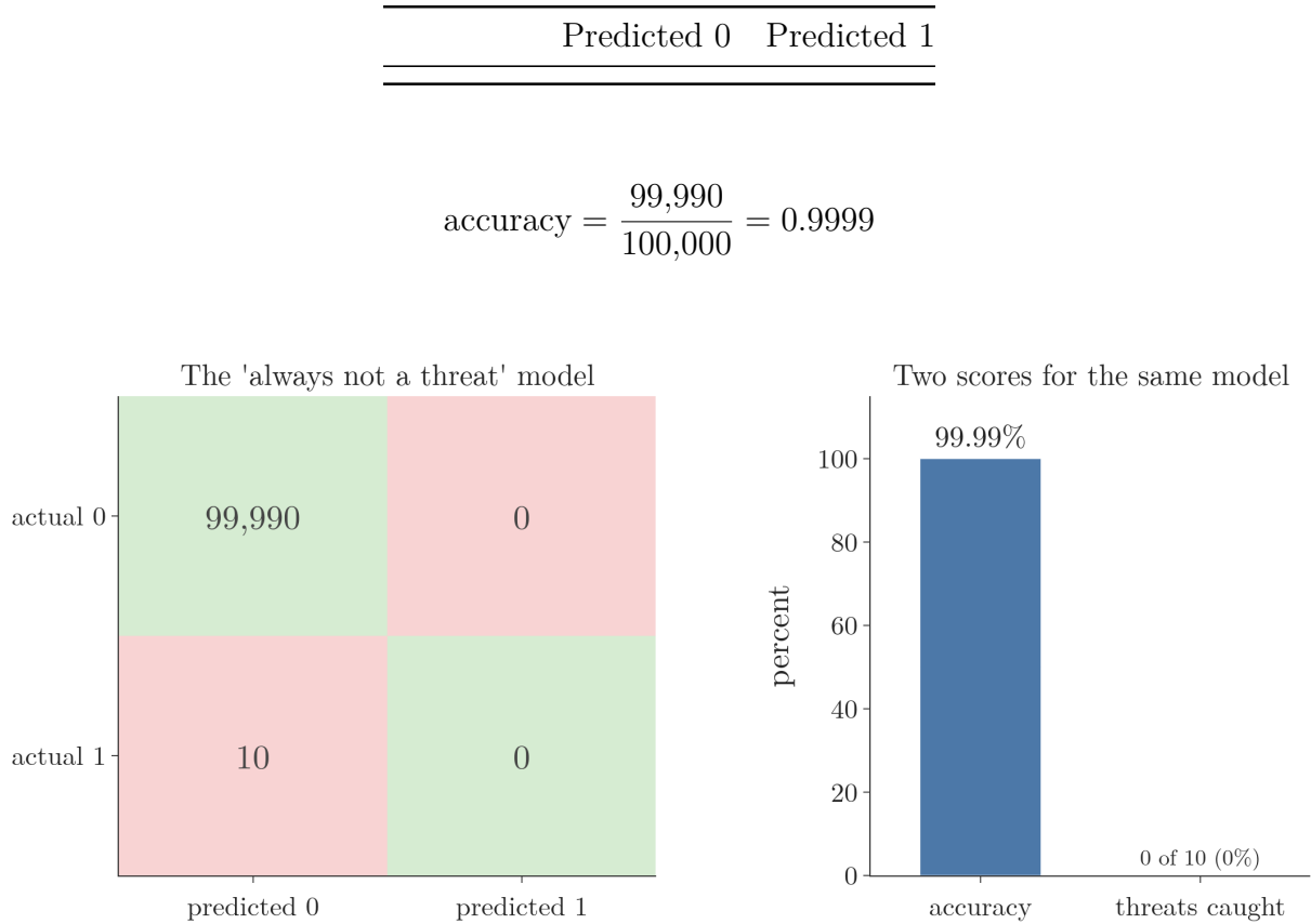
Figure 6: The “always not a threat” model on 100,000 passengers. Left: its confusion matrix. Right: its accuracy against the share of threats it catches.
