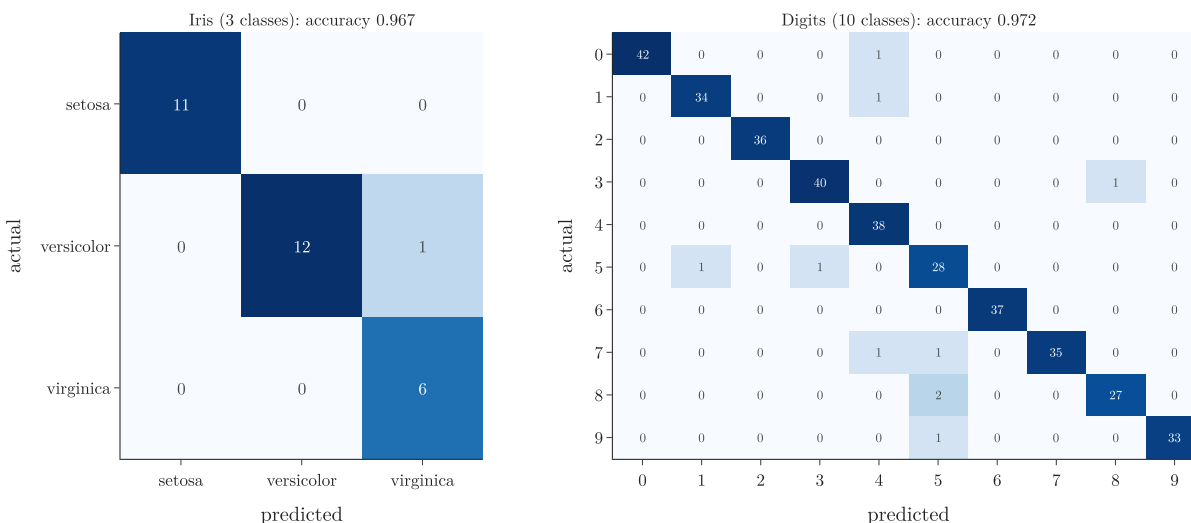
Figure 5: Confusion matrices for iris (3 classes) and digits (10 classes)
