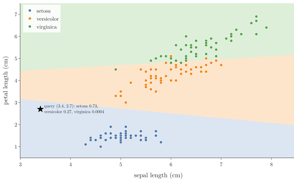
Figure 5: Decision regions of softmax regression on iris
