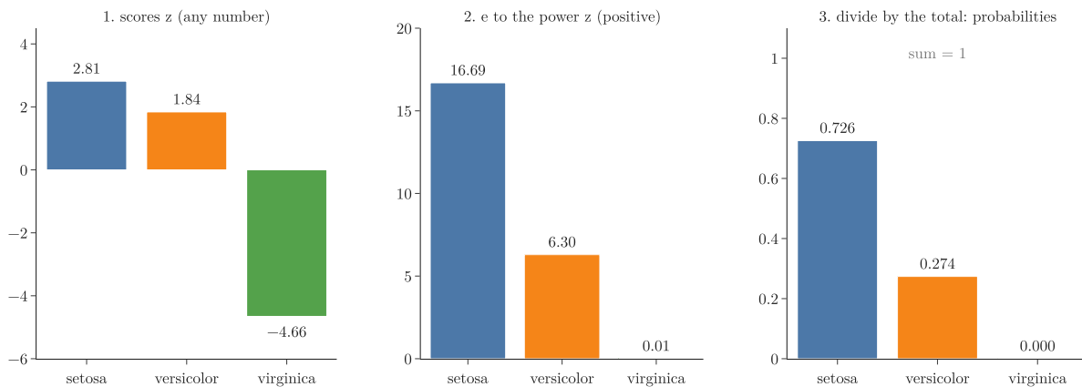
Figure 1: Softmax step by step for one flower
