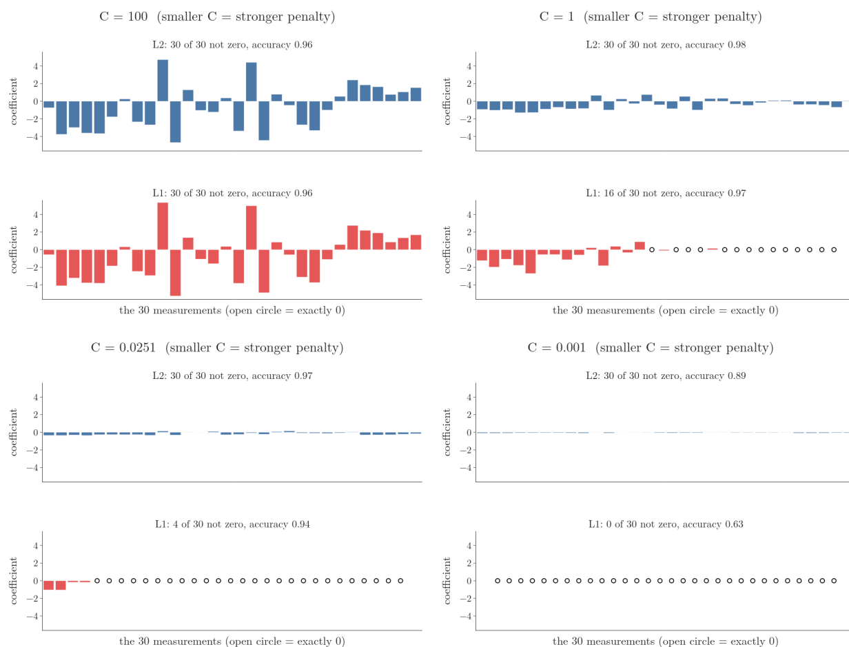
Figure 4: The 30 coefficients on the breast-cancer data as C falls from 100 to 0.001, for L2 (top) and L1 (bottom); titles give the 5-fold CV accuracy
