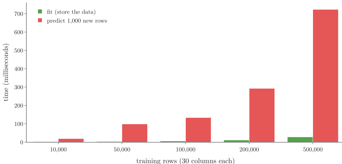
Figure 7: Fit time and prediction time of KNN (brute-force search) as the training set grows
