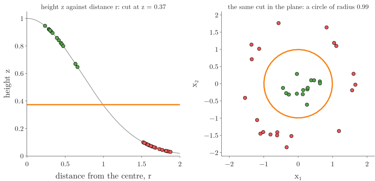
Figure 4: The flat cut of the kernel trick read back in 2D, on the 34 points of Figure 3. Left: height z = e^{-r^2} against the distance r from the centre, with the cut at z = 0.37 (orange). Right: the same cut in the original plane, a circle of radius 0.99 around the green class.
