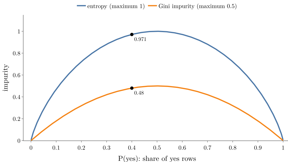
Figure 11: Entropy and Gini impurity against the share of yes observations
