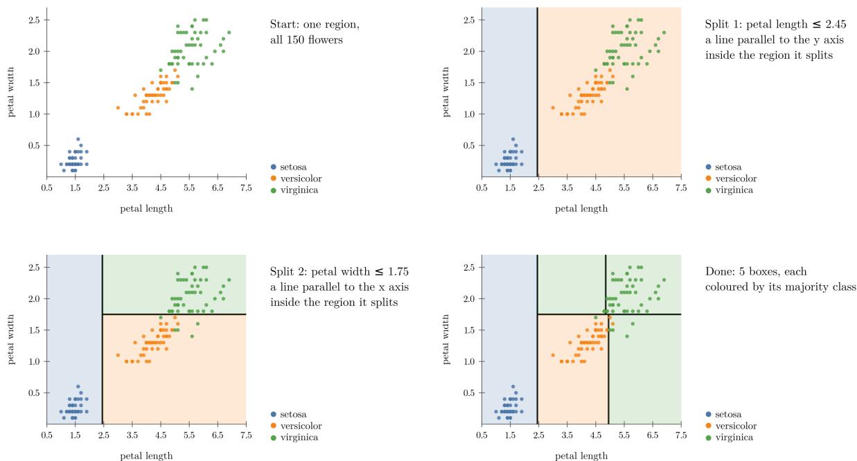
Figure 3: A tree cutting the iris plane, one question at a time
