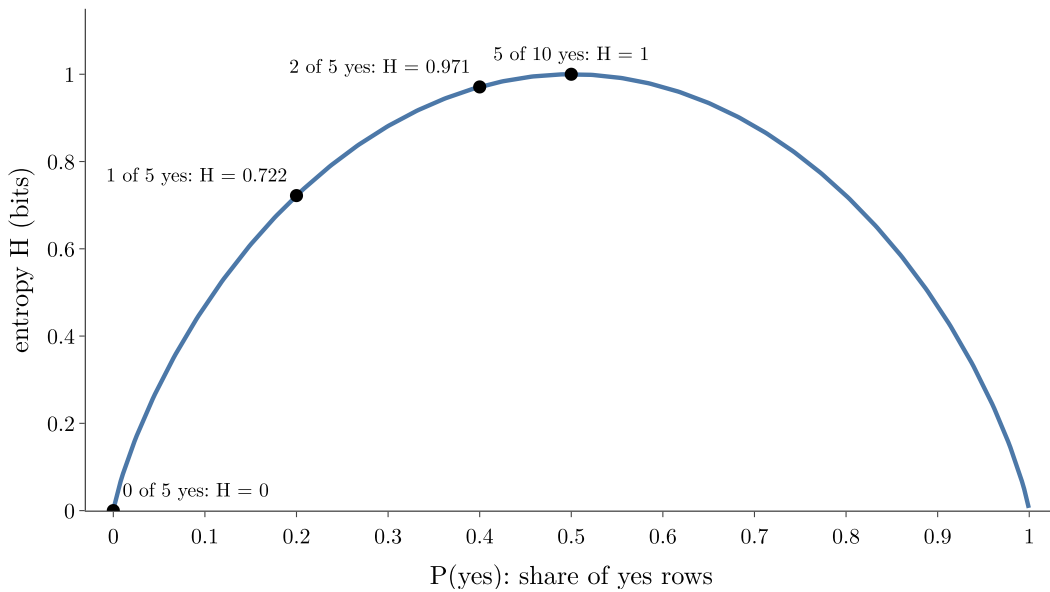
Figure 7: Two-class entropy against the share of yes observations
