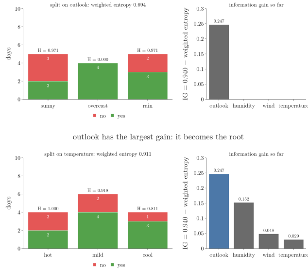
Figure 10: Step 5, one feature per frame: the 14 days split by outlook, humidity, wind and temperature. Bars: each child's yes (green) and no (red) days with its entropy. Right: the information gains so far; outlook's 0.247 is the largest.
