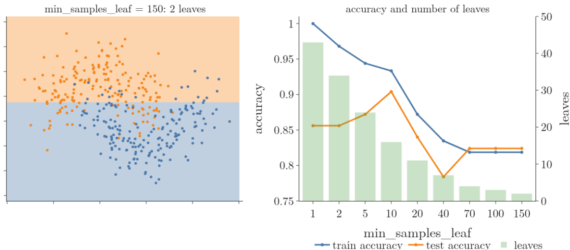
Figure 5: min_samples_leaf from 1 to 150 on the moons data. Left: the decision surface. Right: training accuracy (blue), test accuracy (orange) and the number of leaves (green bars).
