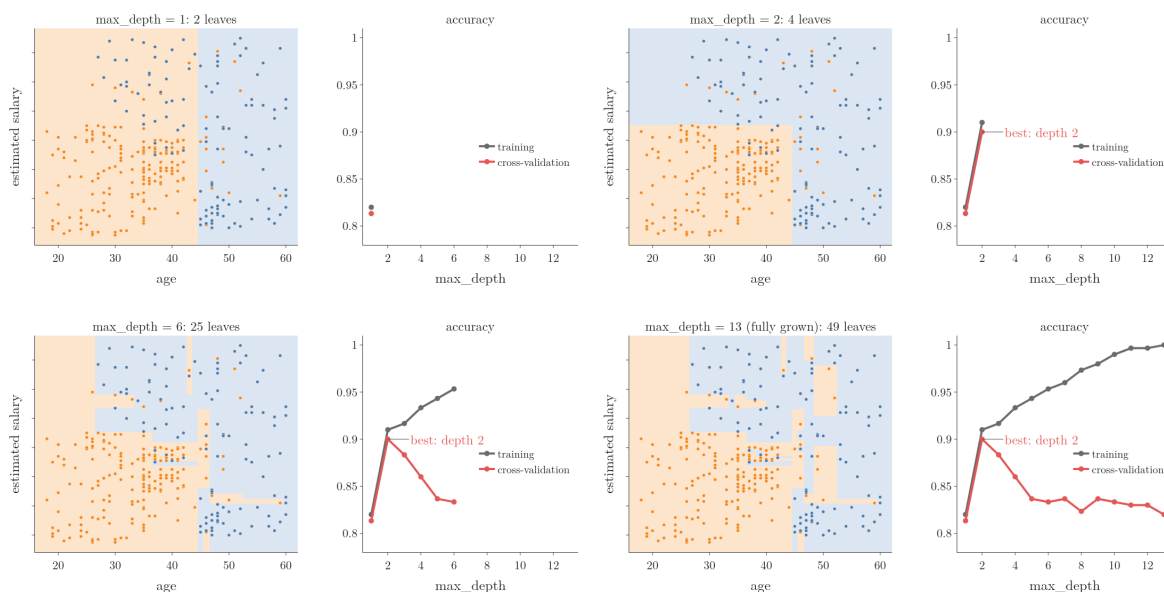
Figure 3: max_depth from 1 to 13 (fully grown) on the Social Network Ads data. Left: the decision surface. Right: training accuracy and 5-fold cross-validation accuracy on the 300 training observations
