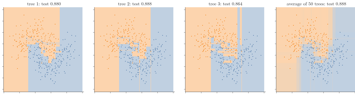
Figure 4: Fully grown trees with max_features = 1 on the moons training data. Three trees with different random seeds draw different surfaces (test accuracy 0.880, 0.888, 0.864); the average vote of 50 such trees (right) scores 0.888.
