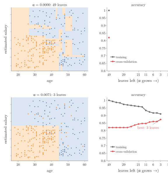
Figure 7: Cost-complexity pruning of the fully grown Social Network Ads tree, one value of \alpha per frame. Left: the decision surface. Right: training accuracy and 5-fold cross-validation accuracy against the number of leaves left. Cross-validation picks the 3-leaf tree.
