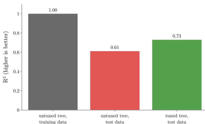
Figure 8: Average R^2 over 20 train-test splits of the California housing data
