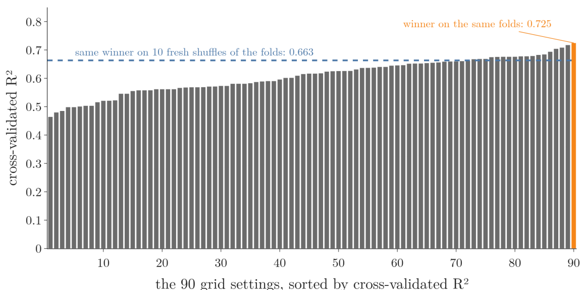
Figure 9: The 90 settings of the Boston grid, sorted by their cross-validated R^2 on the grid’s 5 folds. The winner (orange) scores 0.725; re-scored on 10 fresh shuffles of 5-fold cross-validation, the same setting scores 0.663 (dashed).
