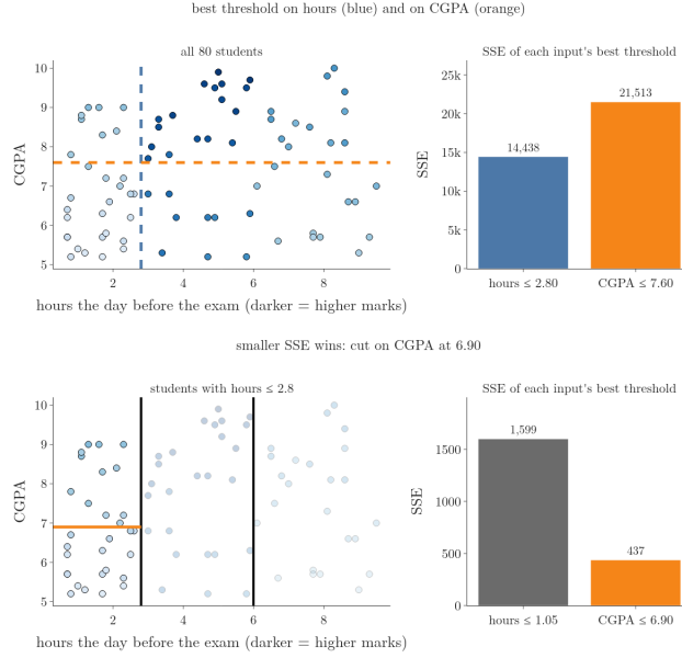
Figure 5: Two inputs competing for each split. Left: the 80 students on the hours-CGPA plane, with the best threshold on hours (blue) and on CGPA (orange) for the current node. Right: the SSE of each; the smaller one makes the cut.
