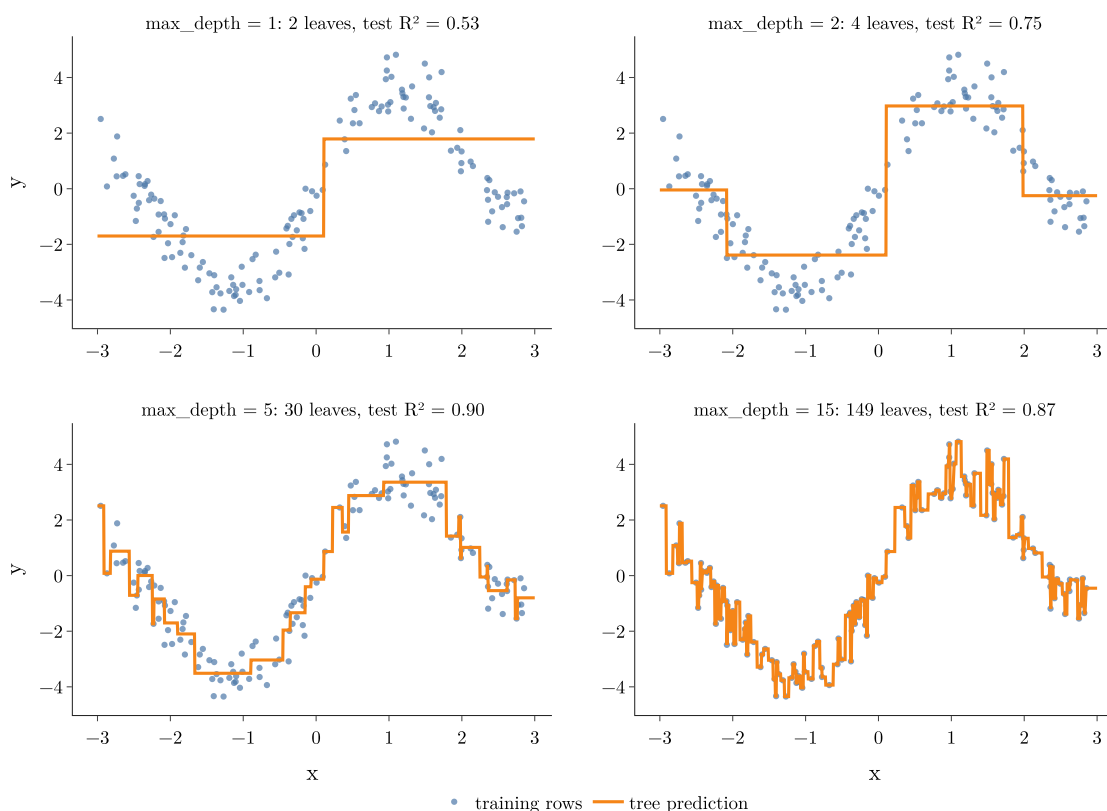
Figure 7: Regression trees of depth 1, 2, 5 and 15 on a noisy wave
