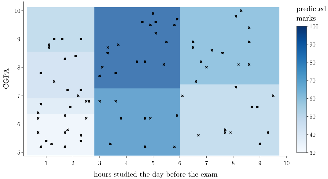
Figure 6: A regression tree with two inputs: each box predicts one mean mark
