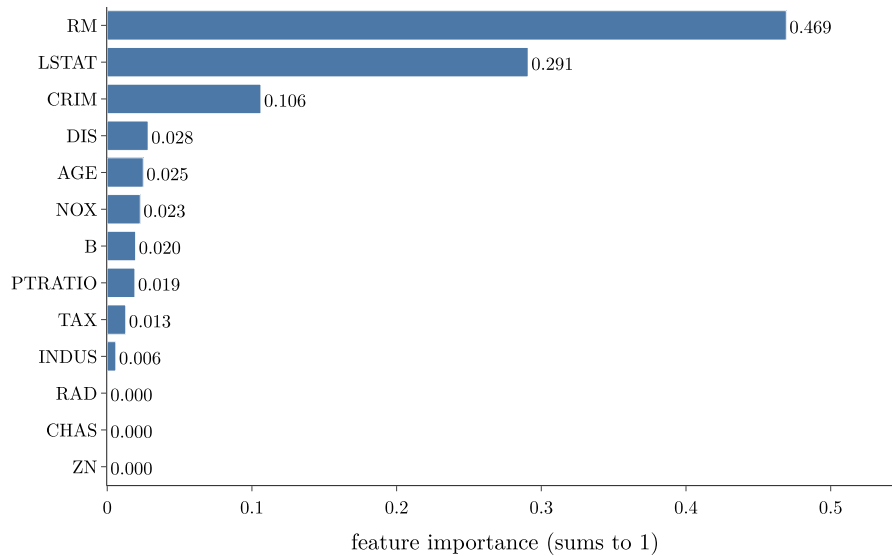
Figure 10: Feature importance of the tuned tree on the Boston data
